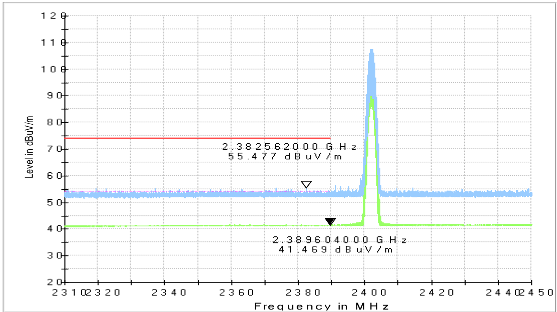
Fig.13. Frequency Band Edges: GFSK, Channel 0, 2.31 GHz – 2.45GHz
