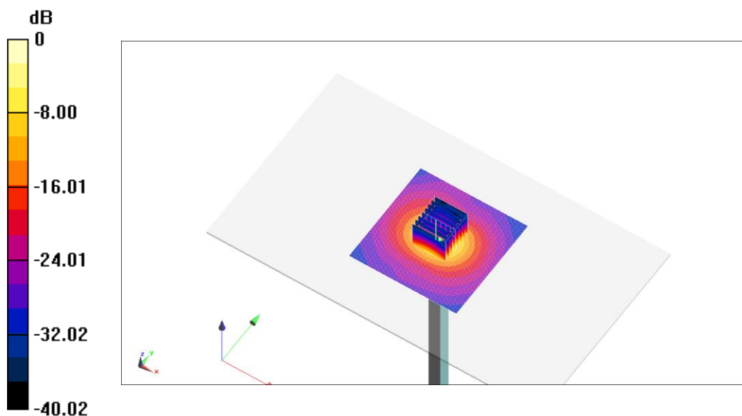
Fig.B.8 validation 5250 MHz 250mW
