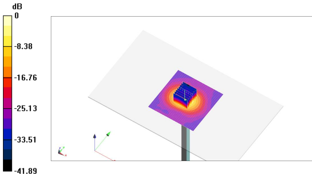
Fig.B.9 validation 5600 MHz 250mW
