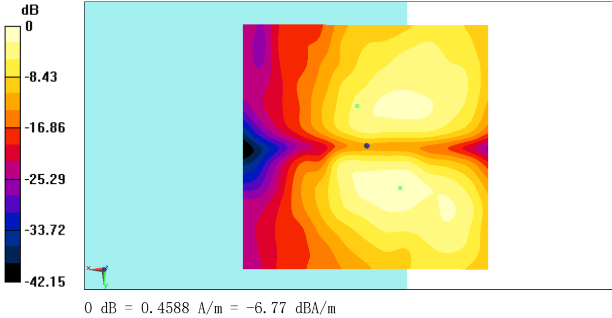
Fig B.13 T-Coil WiFi-5G
