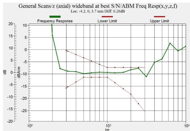
Figure C.3 Frequency Response of CDMA BC10
