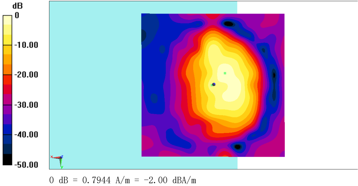
Fig B.14 T-Coil WiFi-5G
