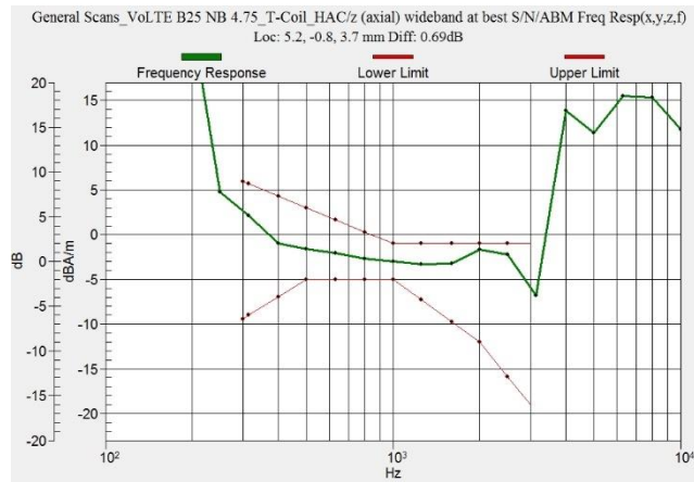
Figure C.4 Frequency Response of LTE B25
