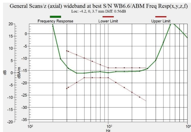
Figure C.6 Frequency Response of WiFi-2.4G
