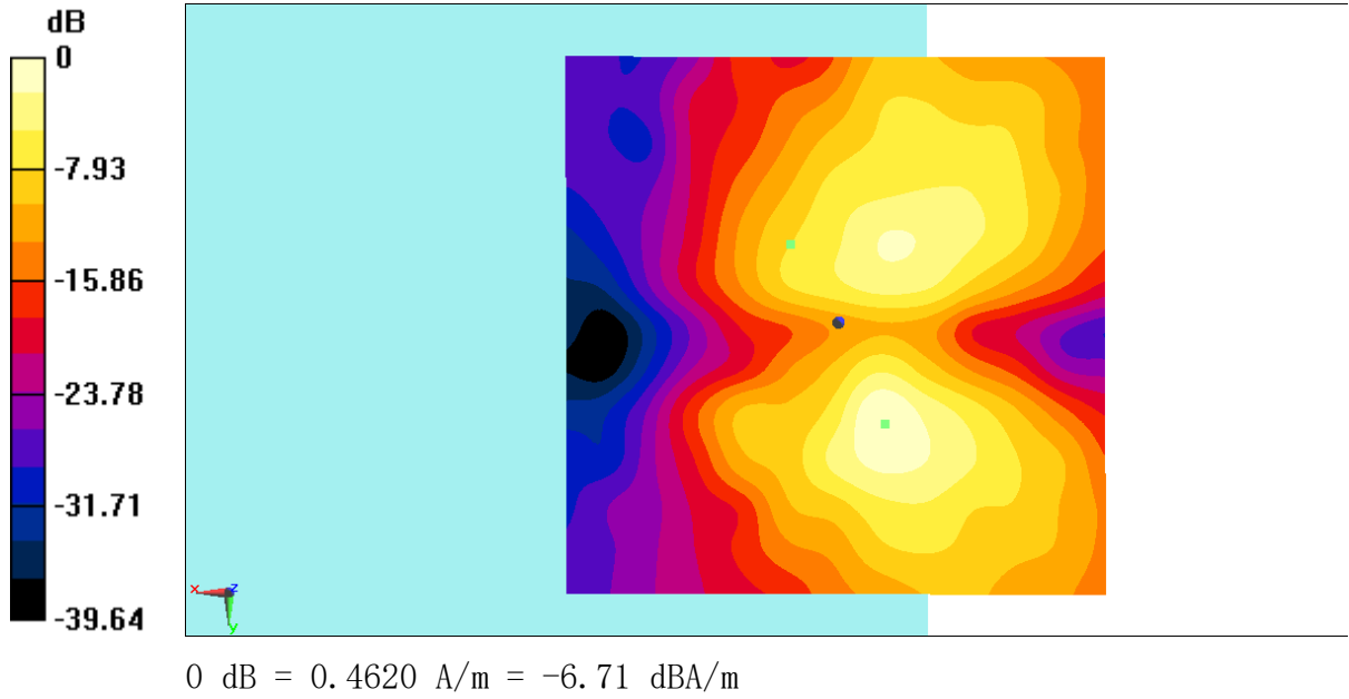
Fig B.11 T-Coil WiFi-2.4G
