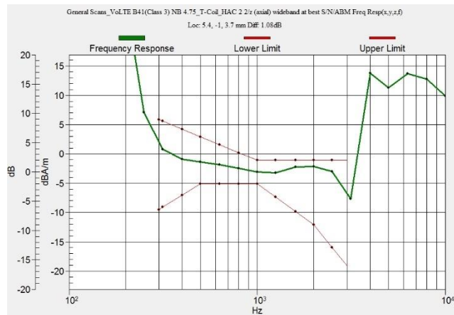
Figure C.5 Frequency Response of LTE B41 PC3
