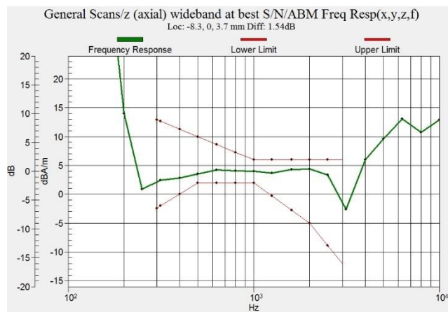
Figure C.9 Frequency Response of LTE B66 - OTT VoIP
