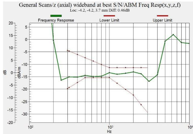
Figure C.7 Frequency Response of WiFi-5G
