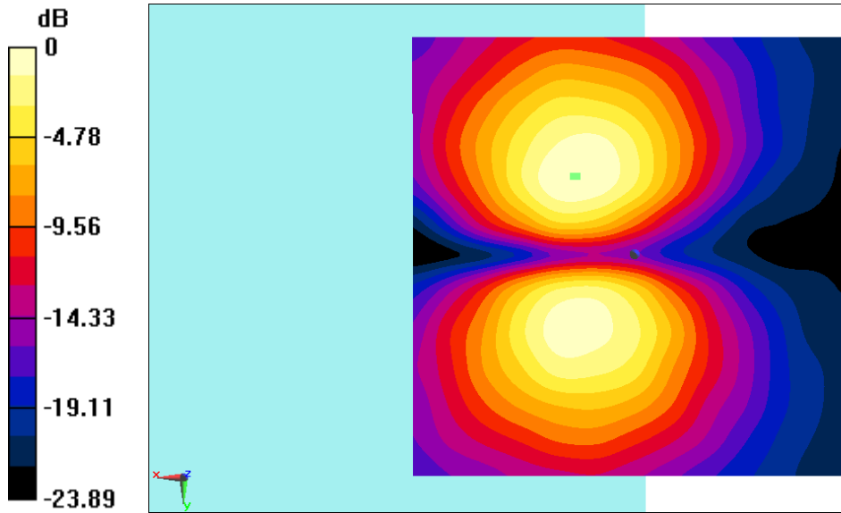
Fig B.7 T-Coil LTE B25
