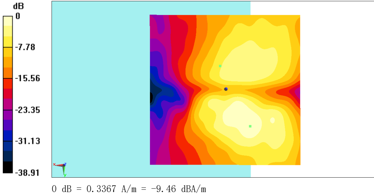
Fig B.5 T-Coil CDMA BC10
