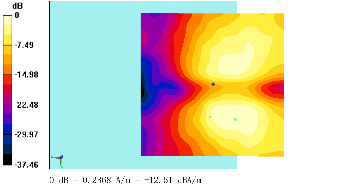
Fig B.21 T-Coil WiFi-2.4G
