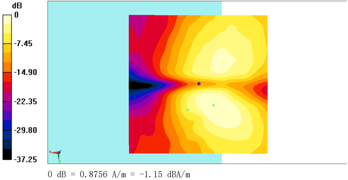
Fig B.19 T-Coil LTE B41
