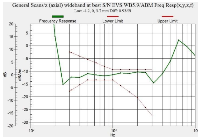
Figure C.11 Frequency Response of WiFi-2.4G - OTT VoIP
