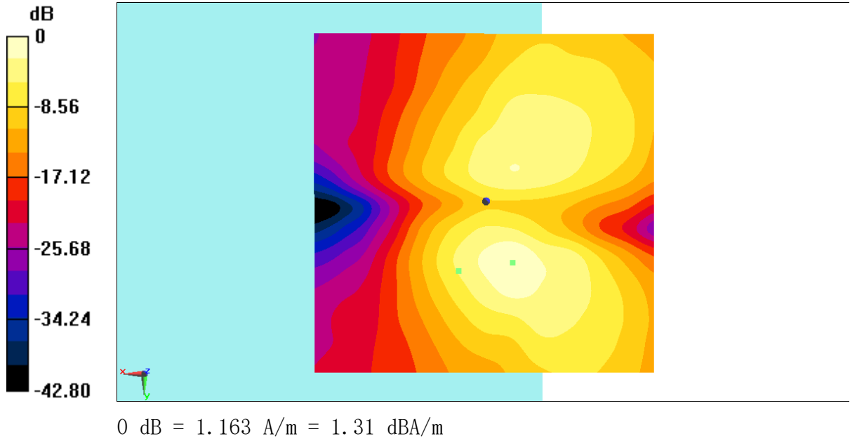
Fig B.17 T-Coil LTE B66
