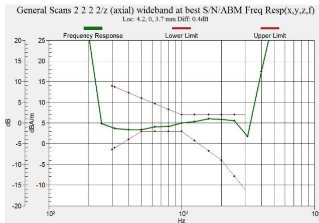
Figure C.12 Frequency Response of WiFi-5G - OTT VoIP
