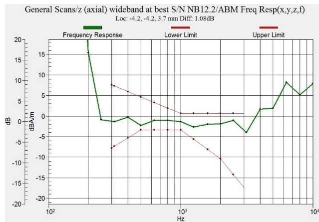
Figure C.8 Frequency Response of CDMA BC1 - OTT VoIP
