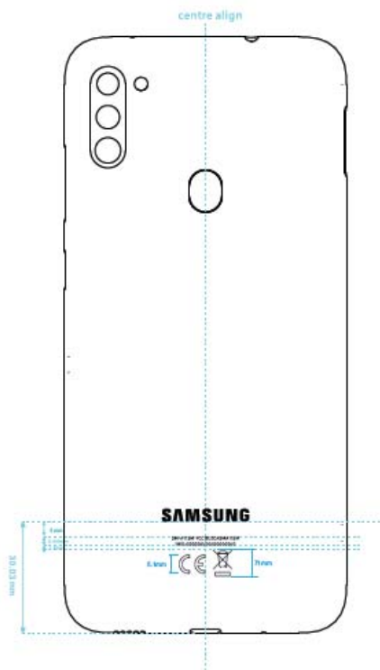
SM-A115M Label:
