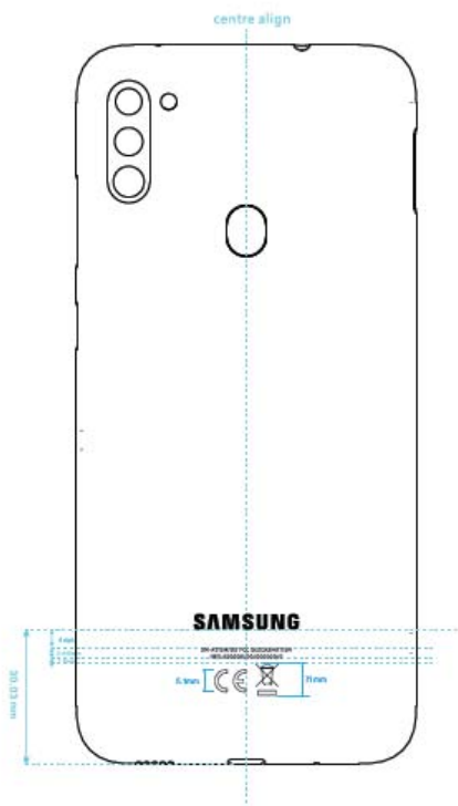
SM-A115M/DS Label:
