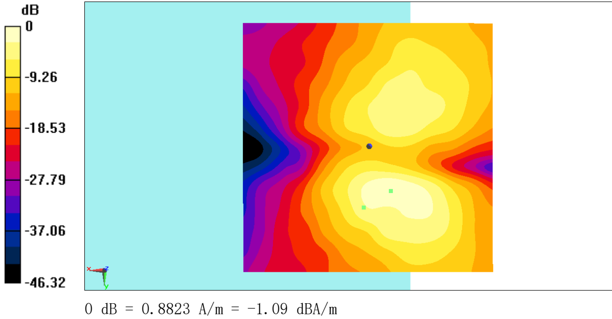
Fig B.15 T-Coil LTE B7
