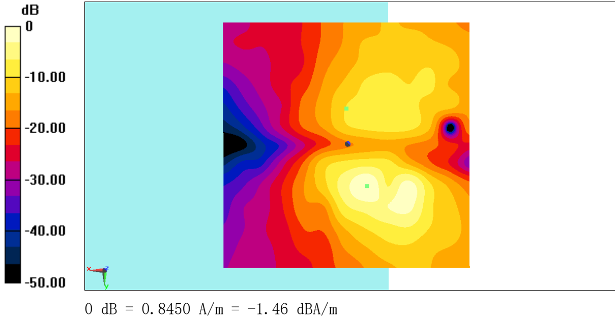
Fig B.21 T-Coil WiFi-5G
