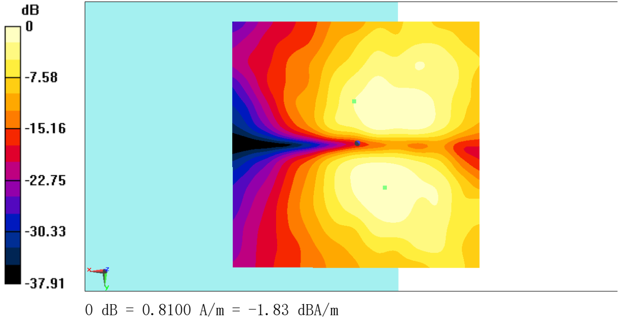
Fig B.17 T-Coil LTE B41
