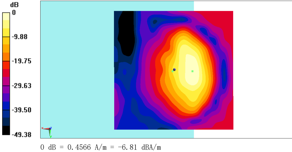
Fig B.12 T-Coil WiFi-5G
