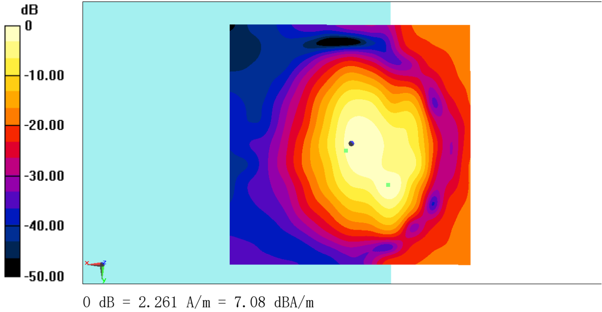
Fig B.16 T-Coil LTE B7
