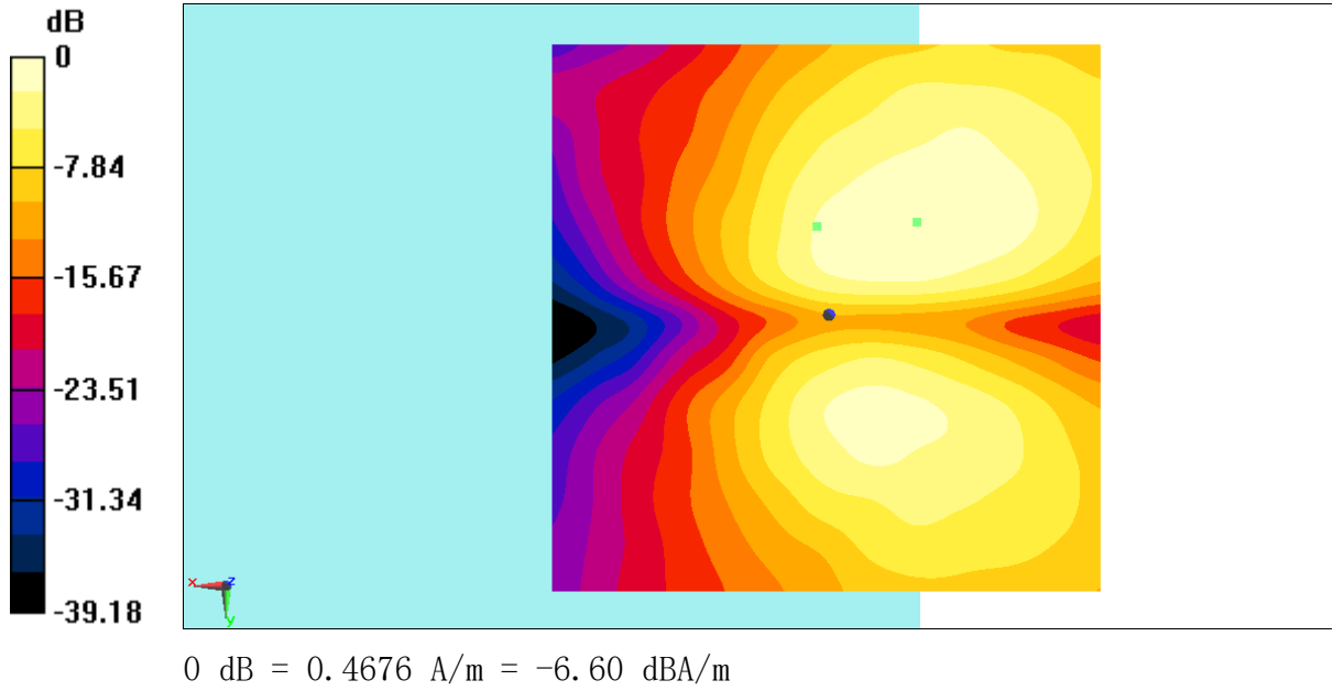
Fig B.7 T-Coil LTE B41
