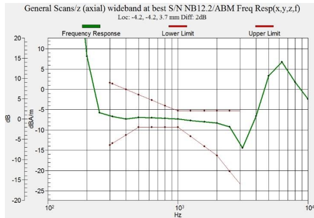
Figure C.8 Frequency Response of LTE B7 - OTT VoIP
