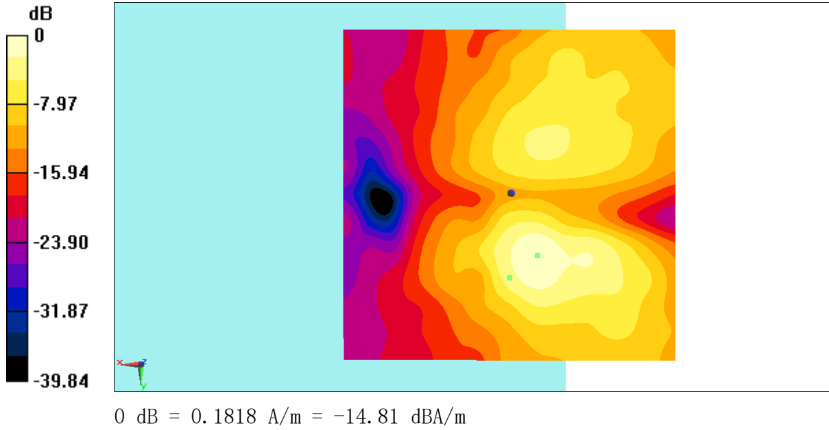
Fig B.11 T-Coil WiFi-5G
