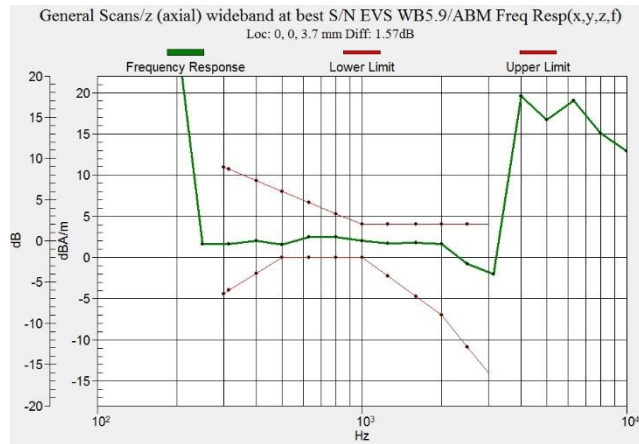
Figure C.7 Frequency Response of WCDMA 850 - OTT VoIP
