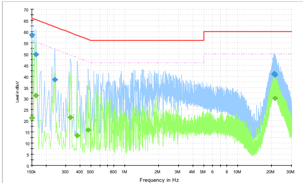
Fig.A.6.1. AC Powerline Conducted Emission-Idle
