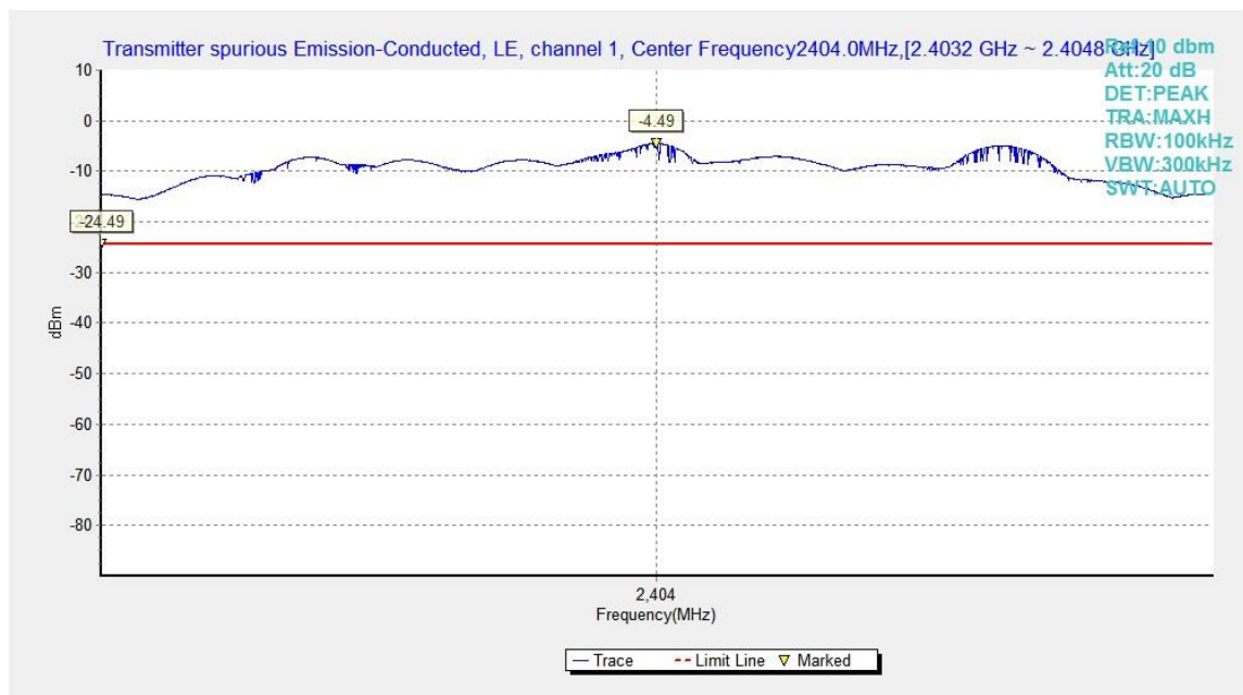
Fig.3. Transmitter Spurious Emission - Conducted: GFSK,2404MHz
