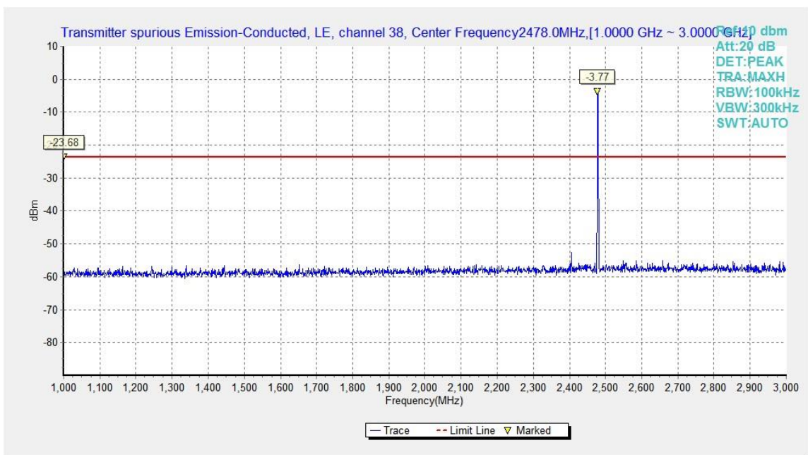
Fig.15. Transmitter Spurious Emission - Conducted: GFSK, 2478 MHz, 1GHz - 3GHz
