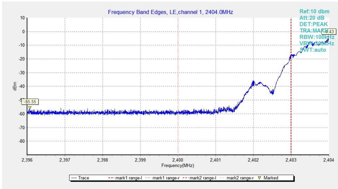
Fig.1. Frequency Band Edges: GFSK, 2404 MHz, Hopping Off
