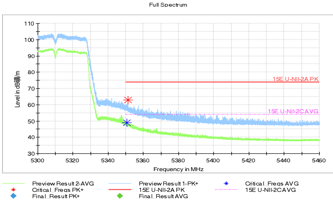
Fig.51 Band Edges (802.11ac-HT40 Ch62, 5310MHz)
