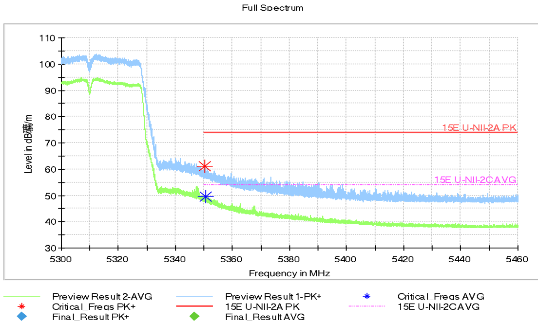
Fig.43 Band Edges (802.11n-HT40 Ch62, 5310MHz)
