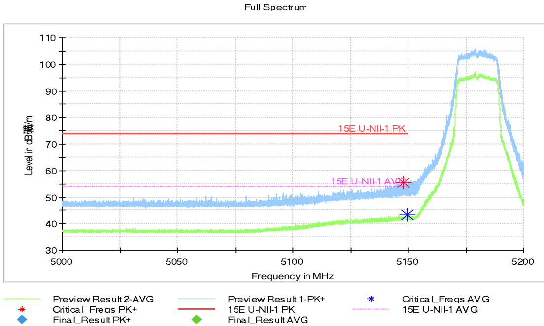
Fig.38 Band Edges (802.11n-HT20 Ch36, 5180MHz)
