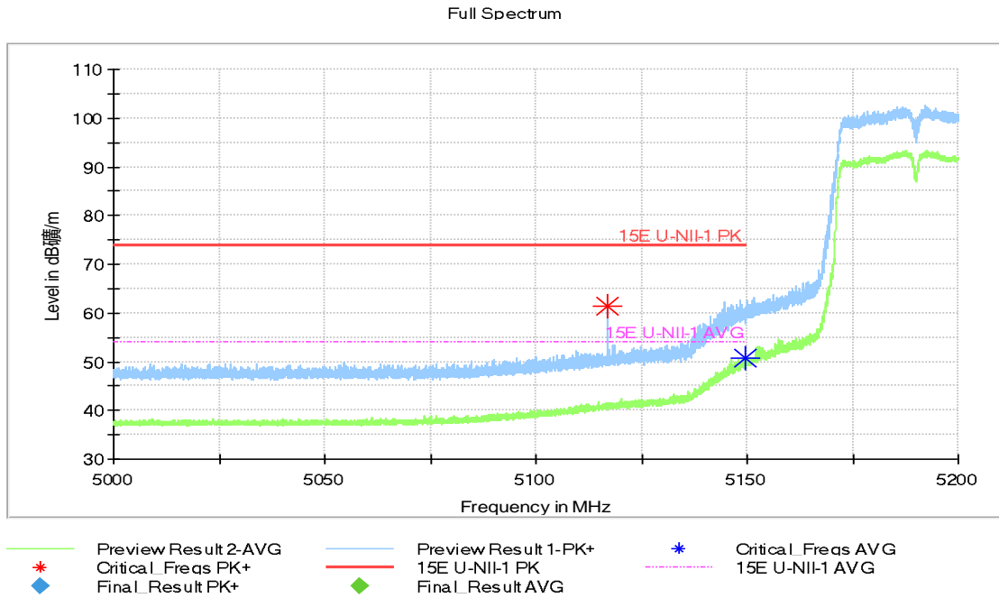
Fig.50 Band Edges (802.11ac-HT40 Ch38, 5190MHz)
