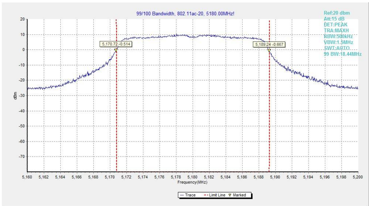
Fig.60 99% Occupied bandwidth (802.11ac-HT20, 5180MHz)
