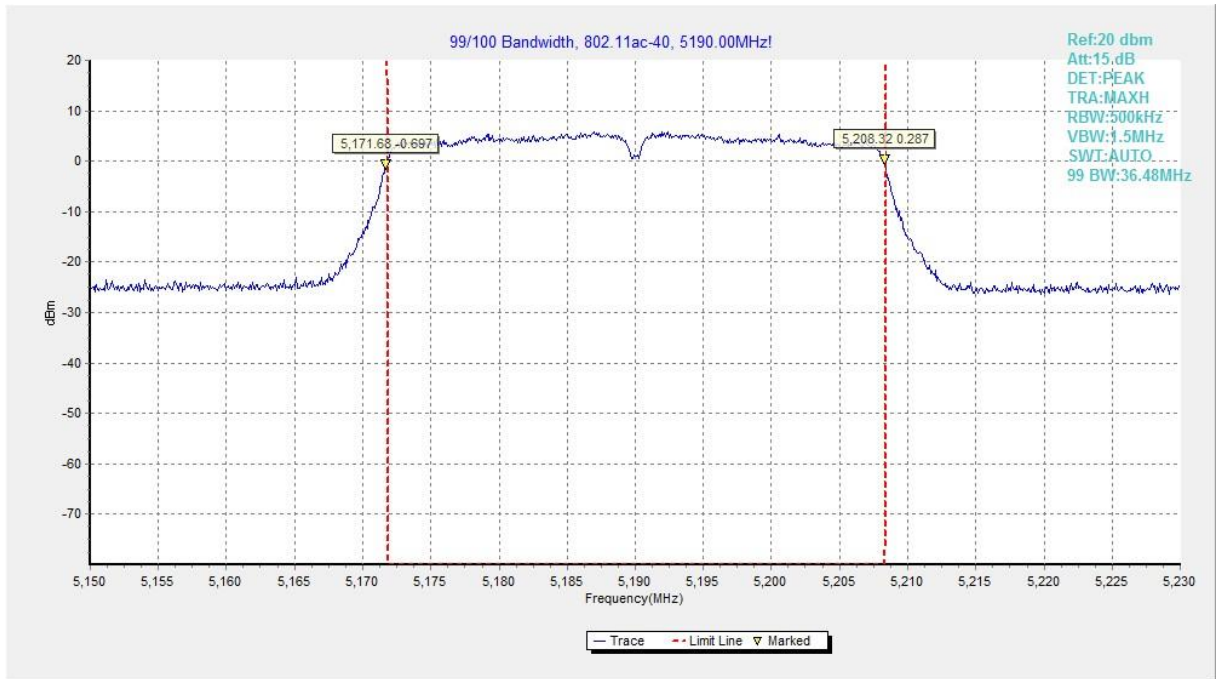
Fig.63 99% Occupied bandwidth (802.11ac-HT40, 5190MHz)
