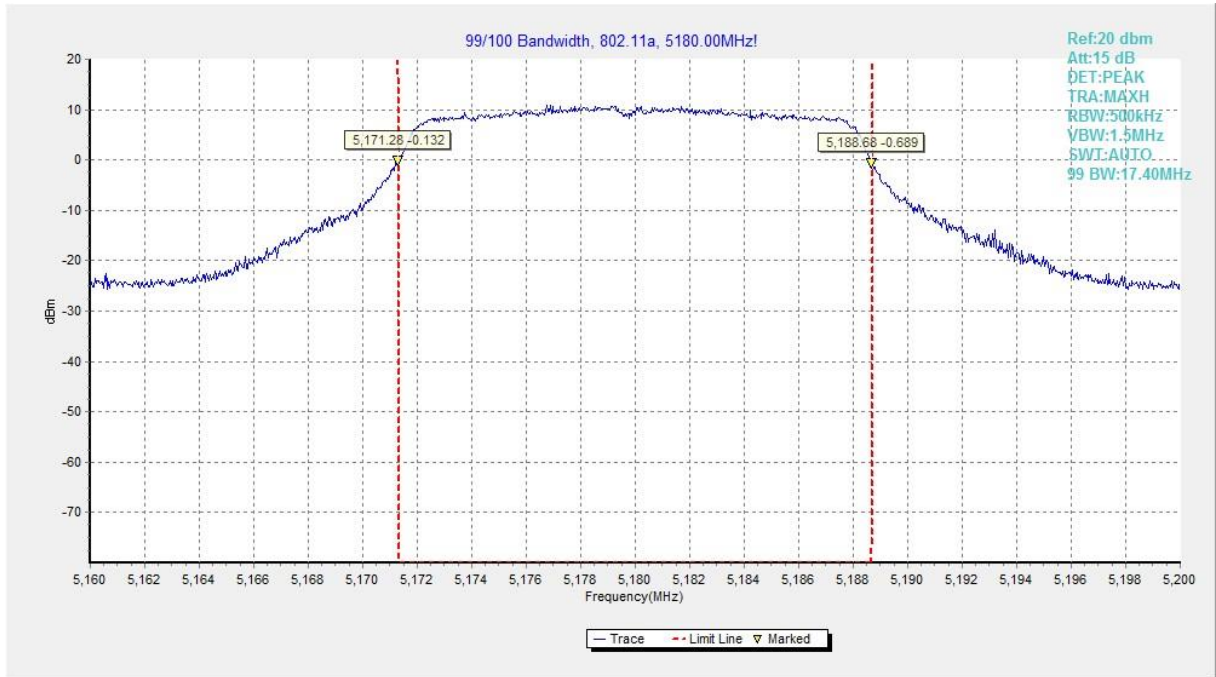
Fig.57 99% Occupied bandwidth (802.11a, 5180MHz)
