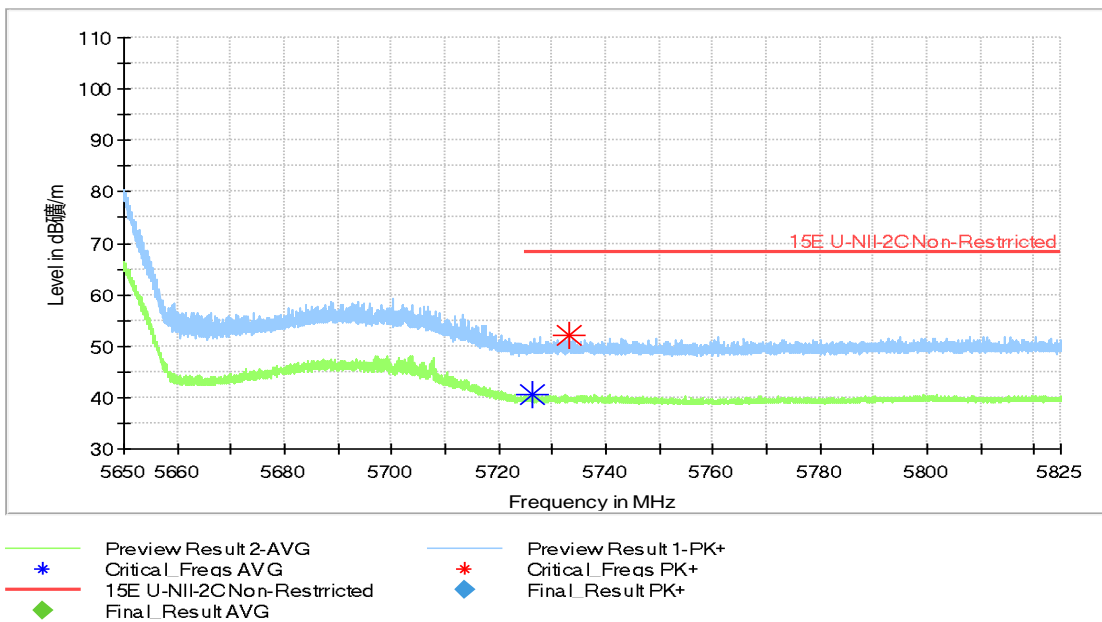
Fig.54 Band Edges (802.11ac-HT80 Ch122, 5610MHz)
