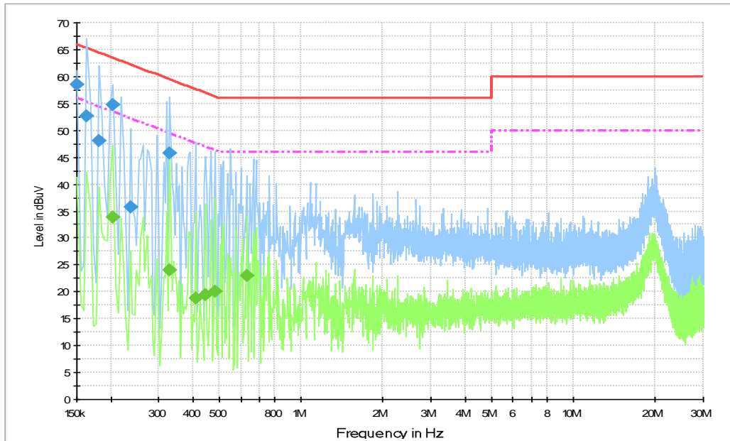
Fig.58 Powerline Conducted Emission-Traffic
