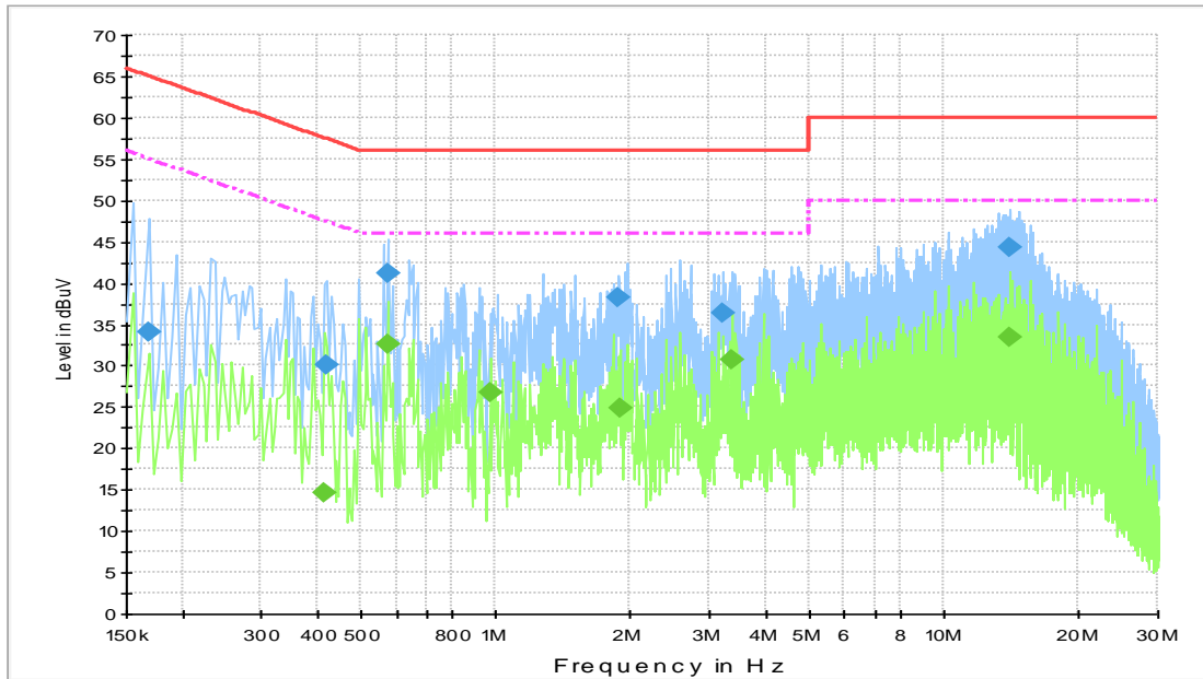
Fig.B.9.1 AC Powerline Conducted Emission- bluetooth
