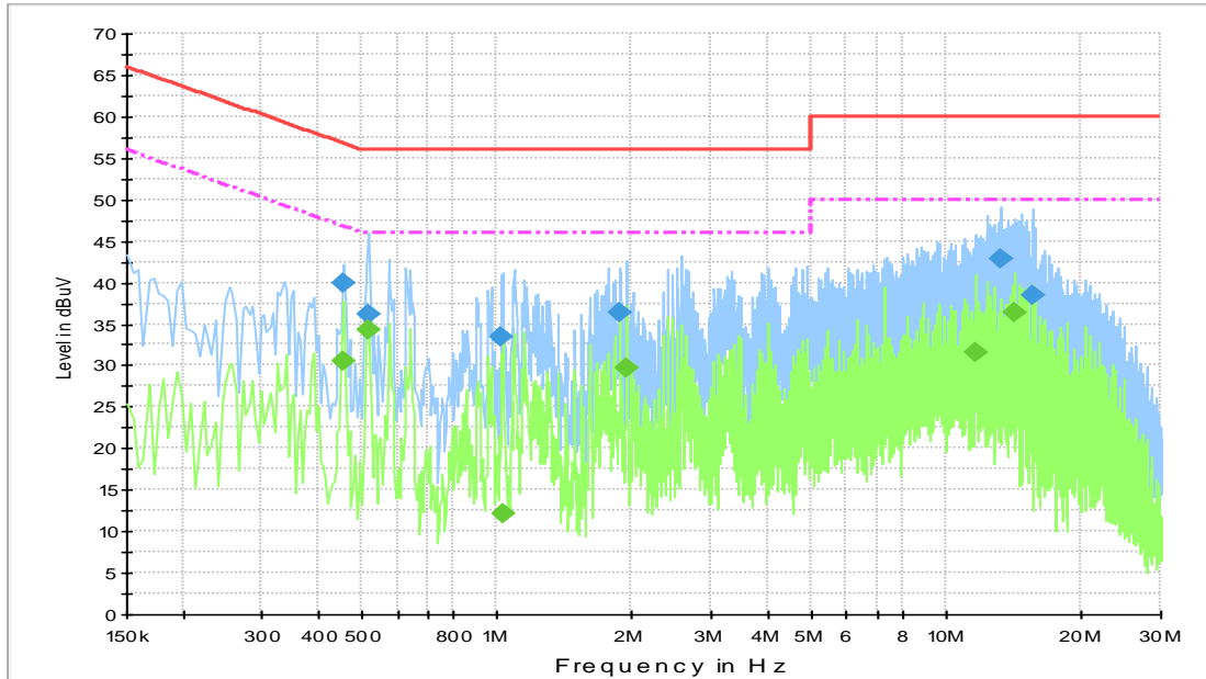
Fig.B.9.2 AC Powerline Conducted Emission-Idle
