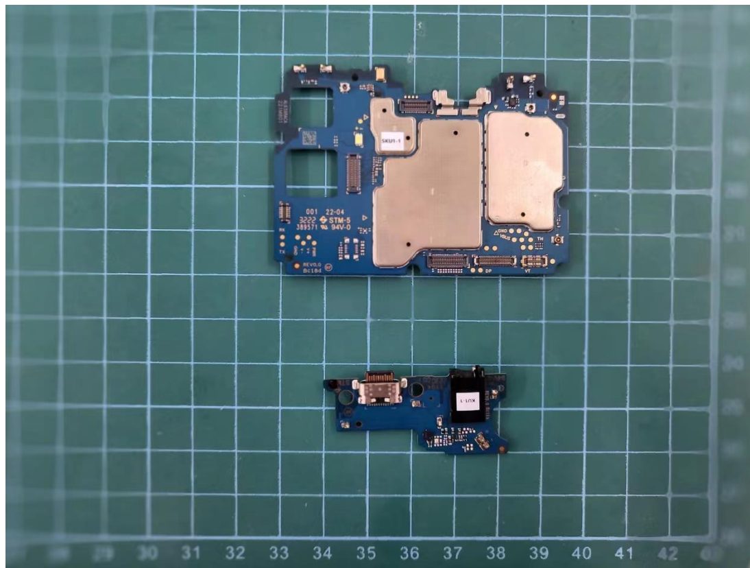
PCB04
