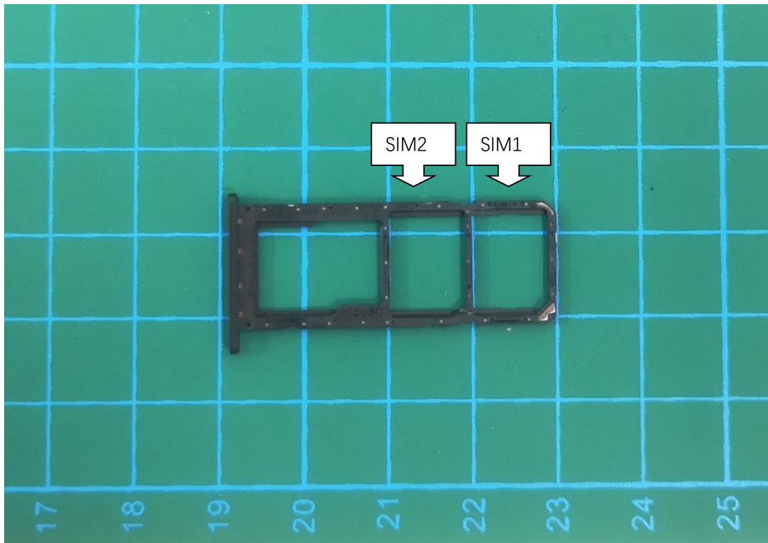
Dual SIM tray for SM-A042M/DS:
