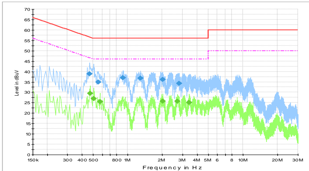
Fig.B.9.1 AC Powerline Conducted Emission- bluetooth
