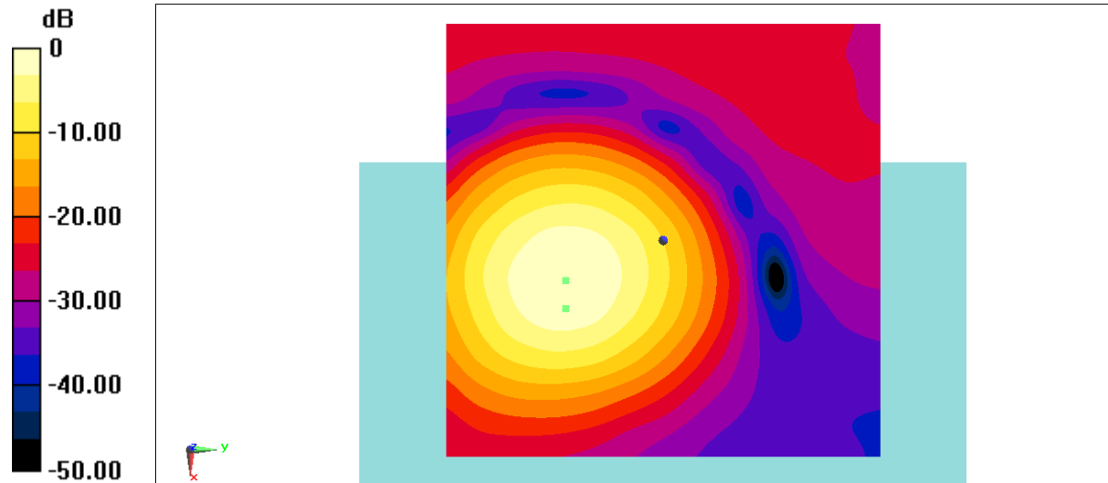
Fig B.2 T-Coil LTE Band41 PC2
