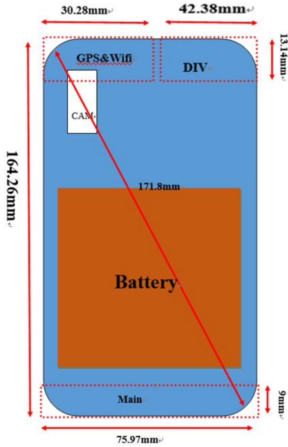
Picture 12 Antenna Locations
