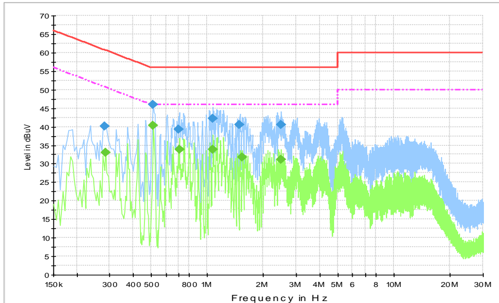
Fig.B.9.2 AC Powerline Conducted Emission-Idle
