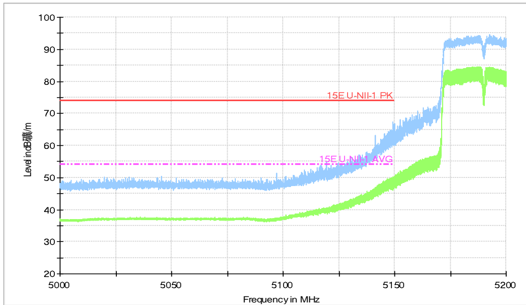
Band Edges (802.11n-HT40 Ch38, 5190MHz)
