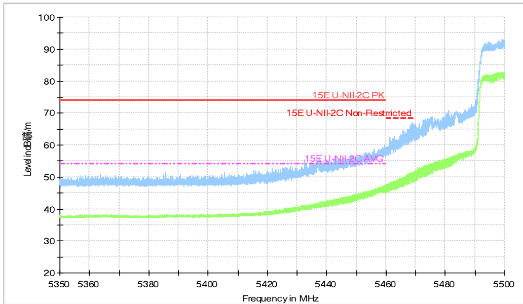
Band Edges (802.11n-HT40 Ch102, 5510MHz)
