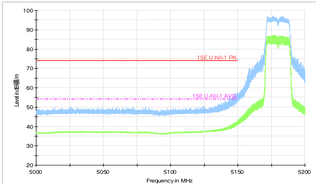
Band Edges (802.11ac-HT20 Ch36, 5180MHz)
