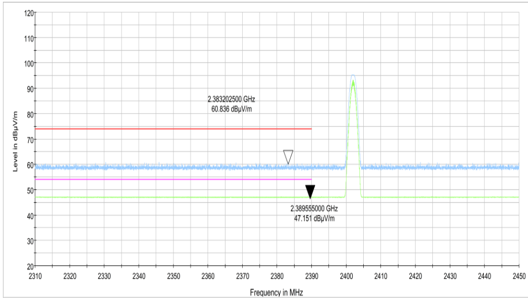
Fig.3. Frequency Band Edges: GFSK, 2402 MHz, 2.31 GHz – 2.45GHz
