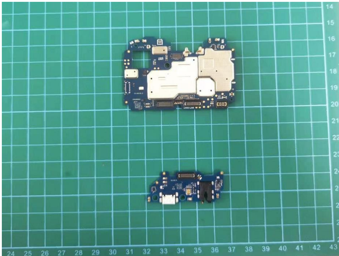
PCB04
