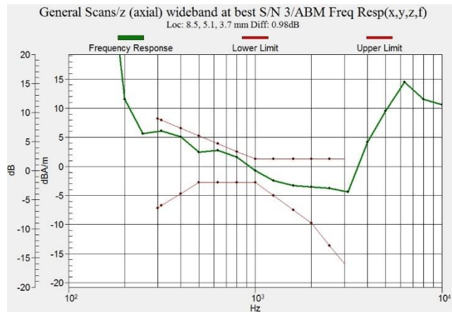
Figure C.2 Frequency Response of LTE B7
