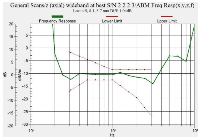
Figure C.5 Frequency Response of CDMA10 - OTT VoIP
