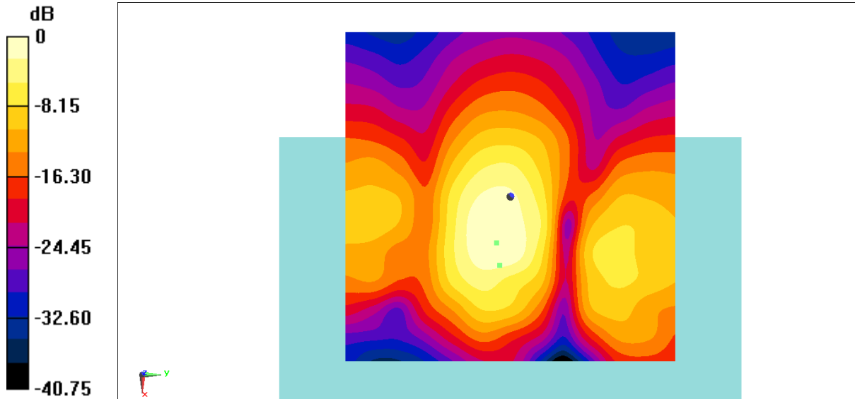
Fig B.5 T-Coil LTE B41
