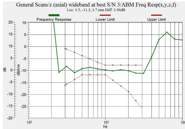
Figure C.7 Frequency Response of LTE B41 PC2 – OTT VoIP
