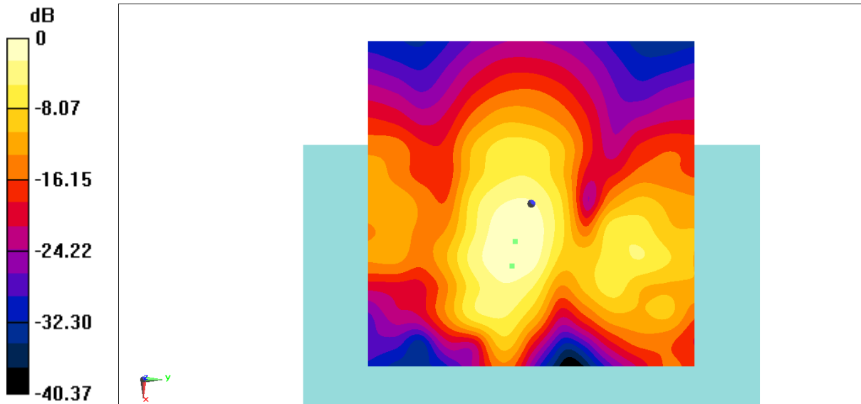
Fig B.3 T-Coil LTE B7
