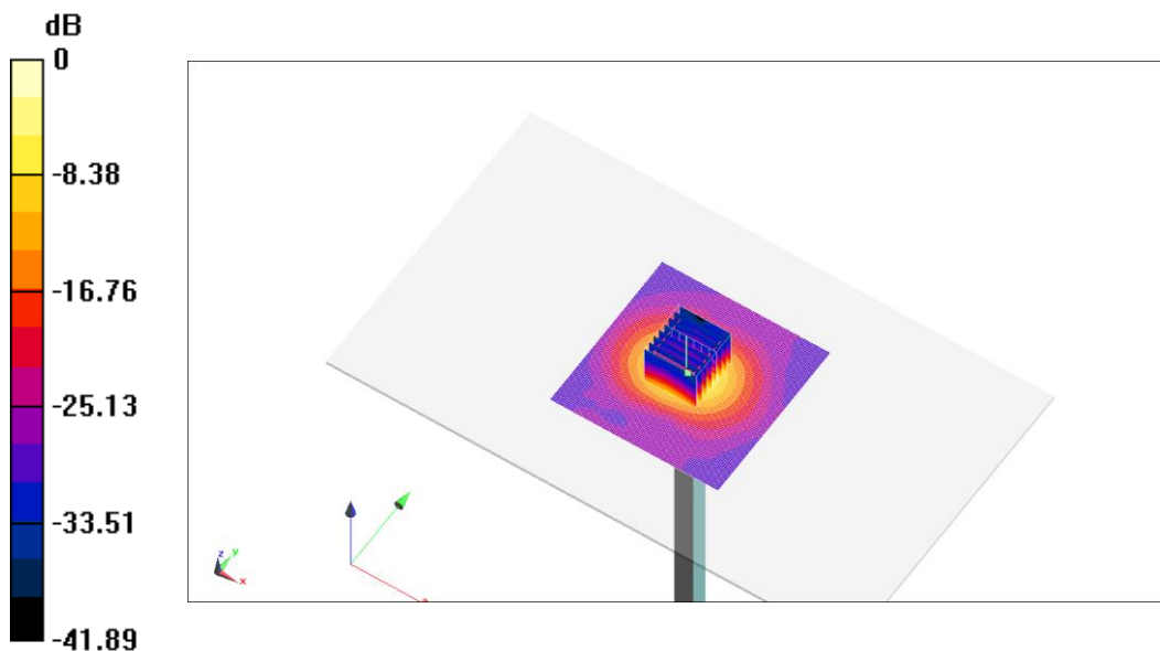
Fig.B.11 validation 5600 MHz 250mW
