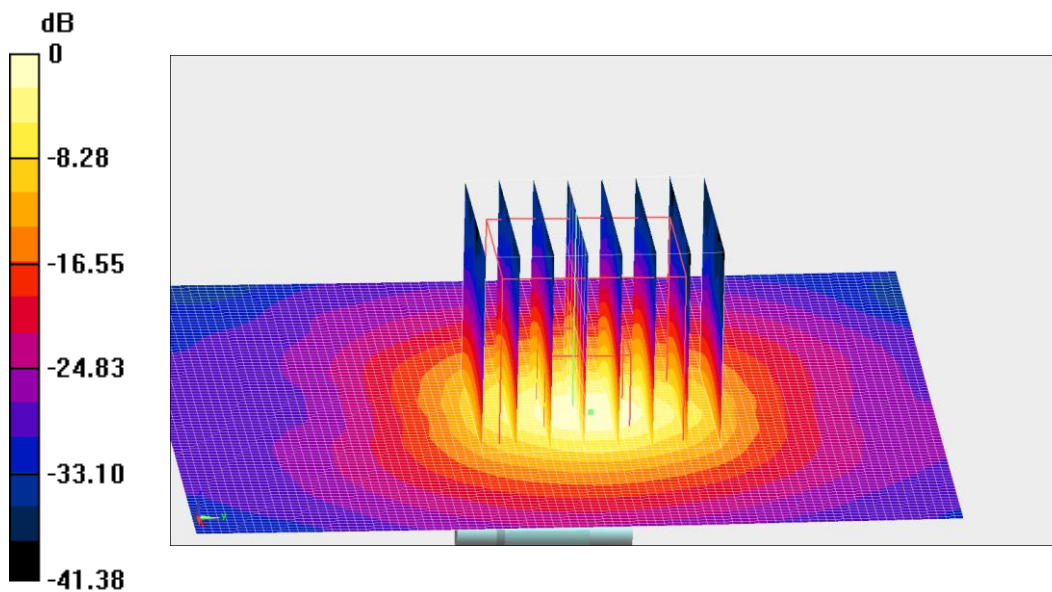
Fig.B.12 validation 5750 MHz 250mW
