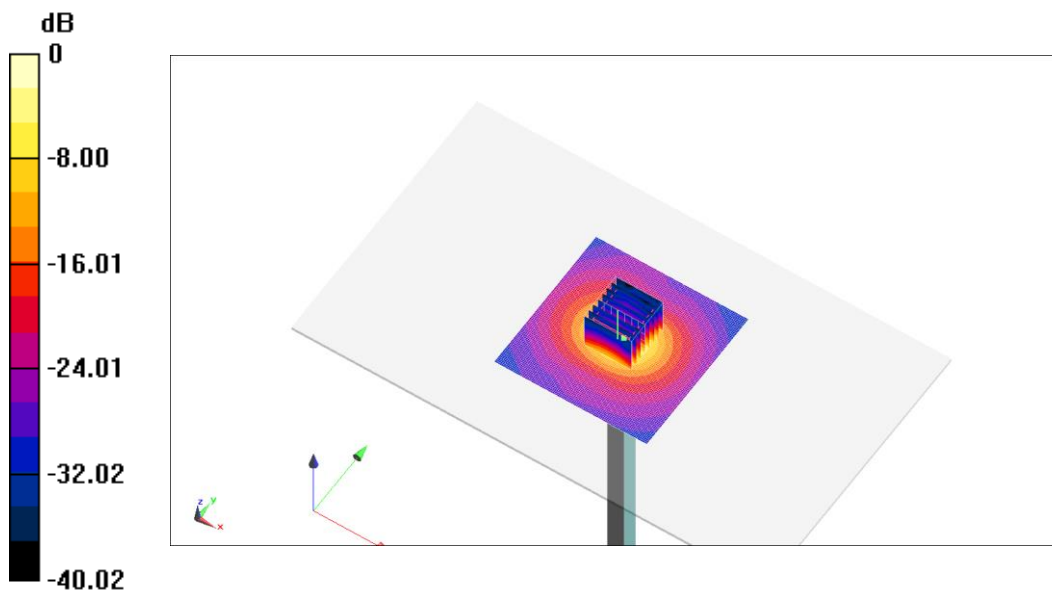
Fig.B.10 validation 5250 MHz 250mW
