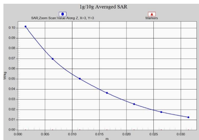
Fig. 1-23 Z-Scan at power reference point (LTE B66 Body)
