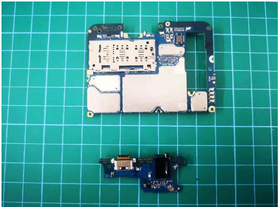
PCB04
