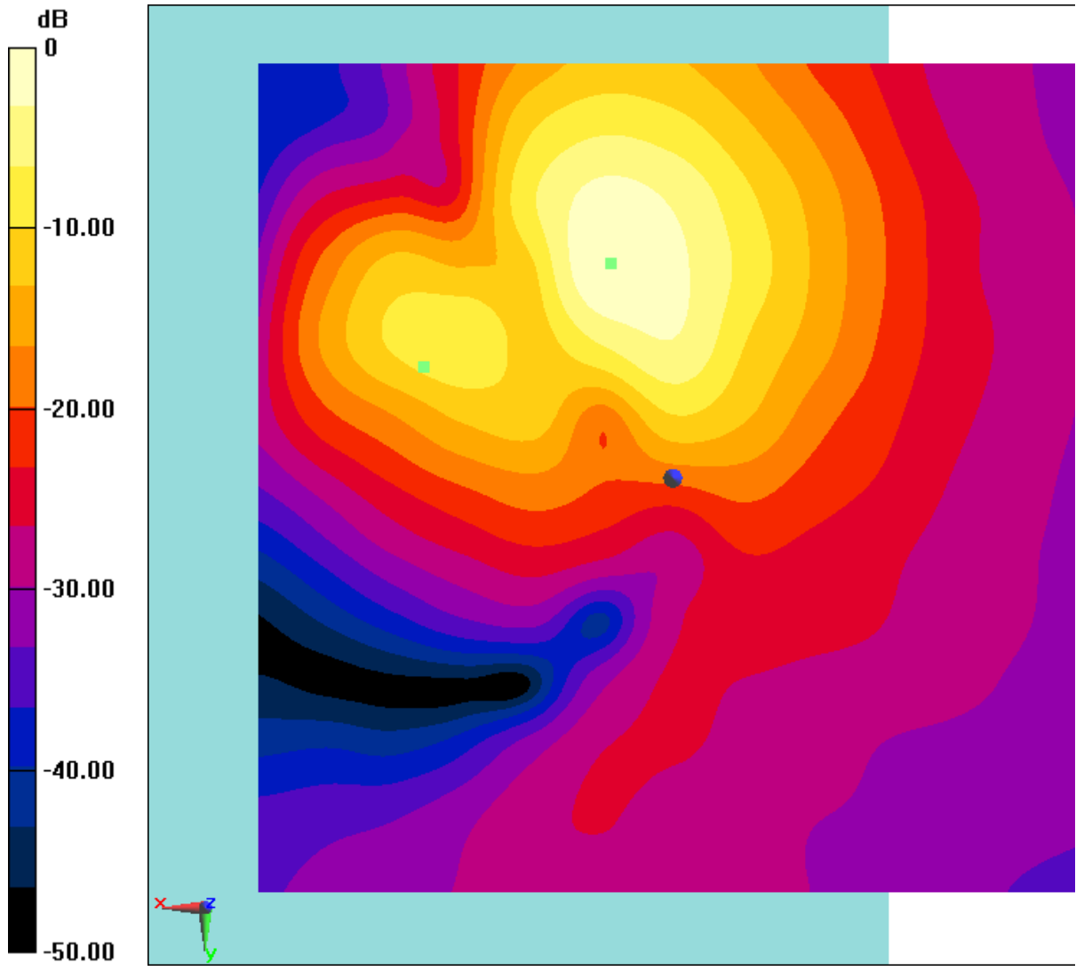
Fig B.16 T-Coil LTE B7
