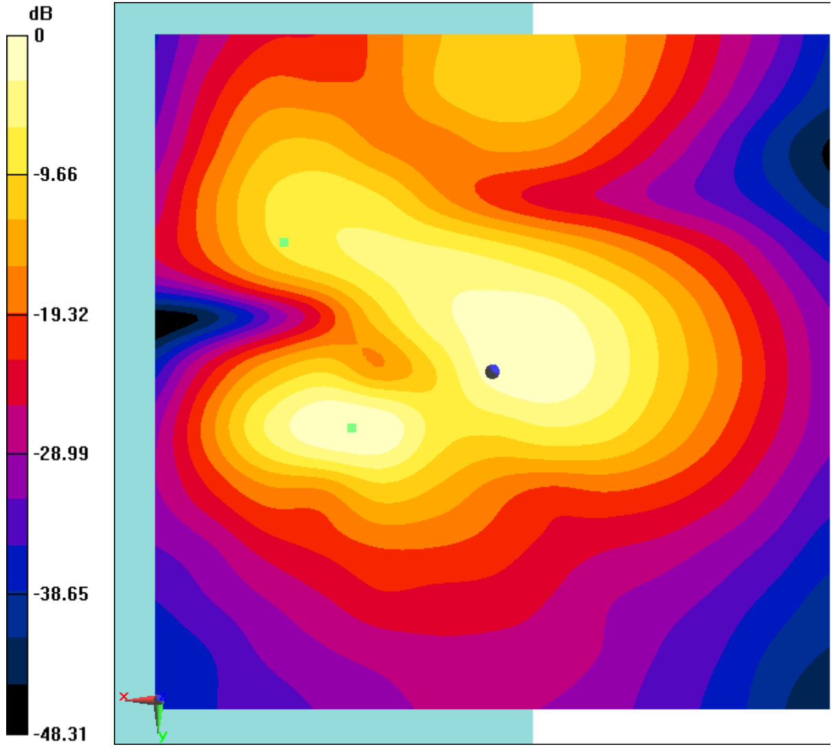
Fig B.29 T-Coil LTE B2
