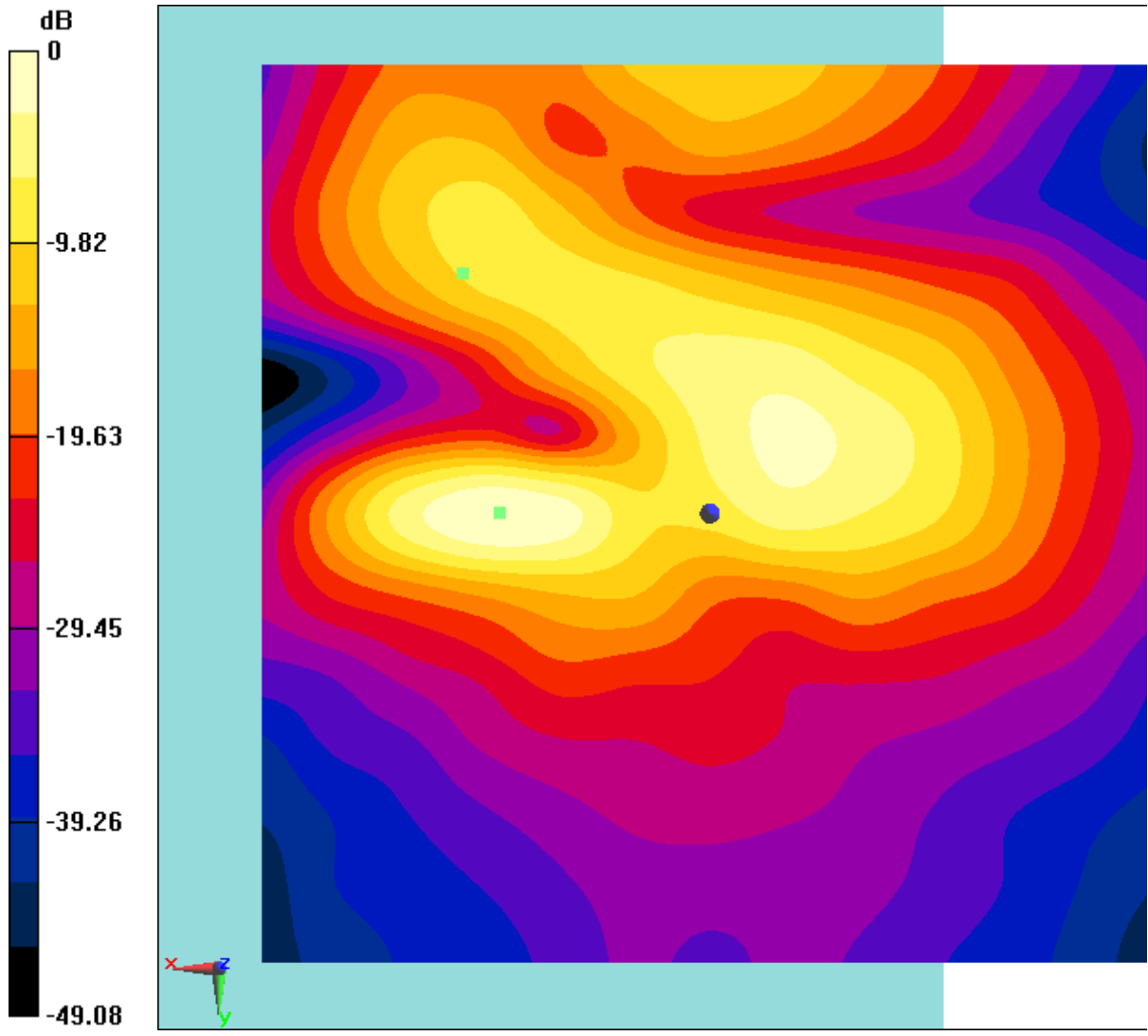
Fig B.15 T-Coil LTE B7
