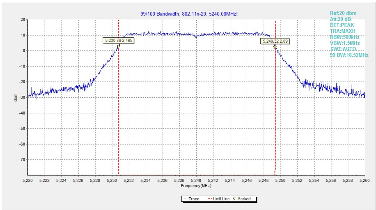
Fig.54 99% Occupied bandwidth (802.11n-HT20, 5240MHz)
