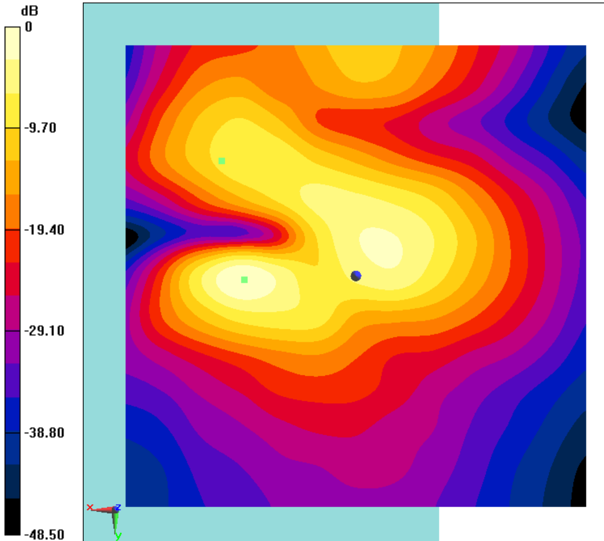
Fig B.11 T-Coil LTE B2
