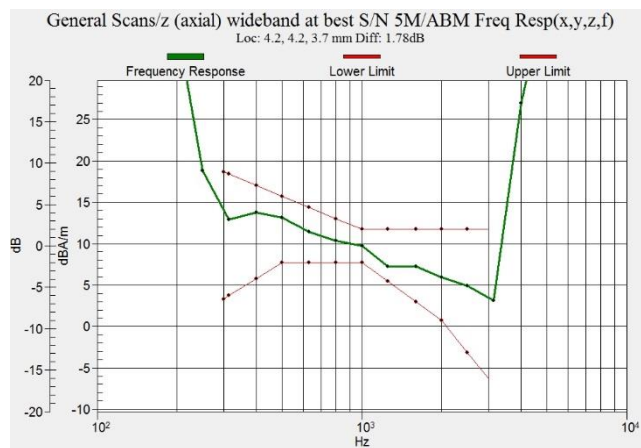
Figure C.15 Frequency Response of LTE B2 - OTT VoIP
