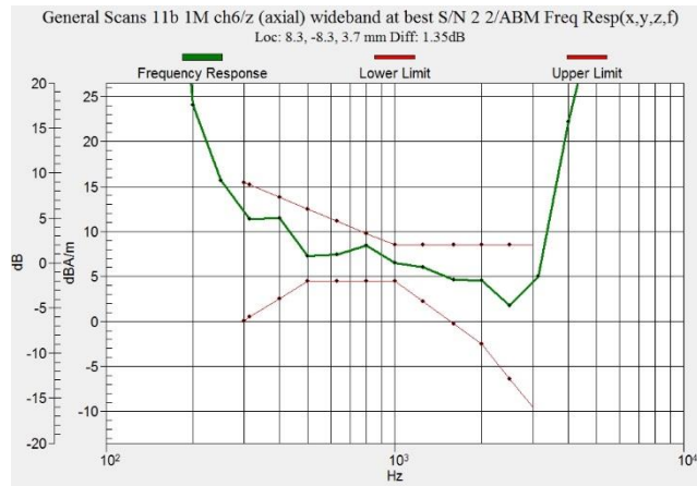
Figure C.16 Frequency Response of WiFi-2.4G - OTT VoIP
