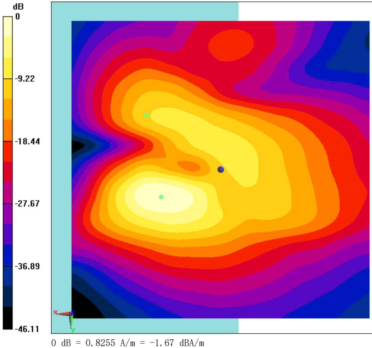
Fig B.1 T-Coil GSM 850
