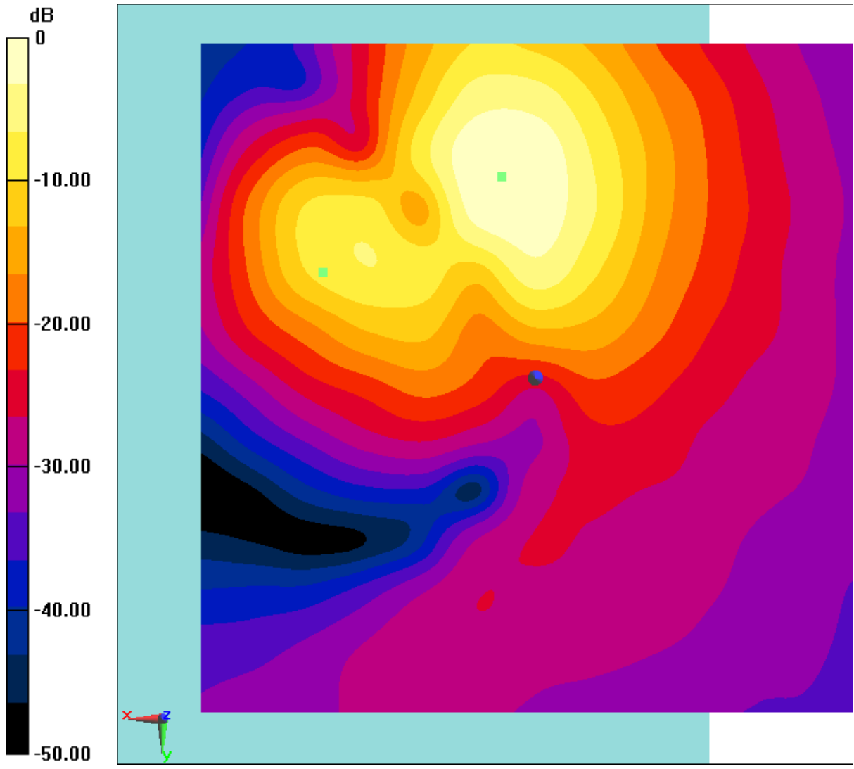
Fig B.20 T-Coil LTE B66
