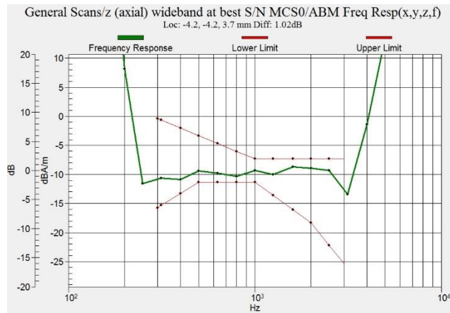
Figure C.17 Frequency Response of WiFi-5G - OTT VoIP
