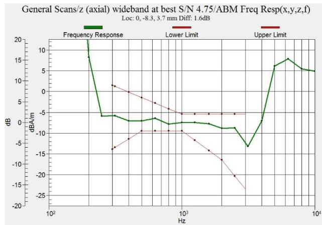
Figure C.14 Frequency Response of W1900 - OTT VoIP
