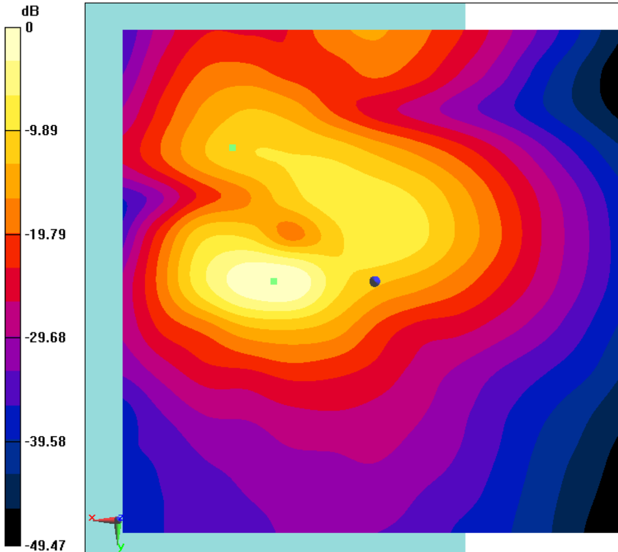
Fig B.21 T-Coil LTE B71
