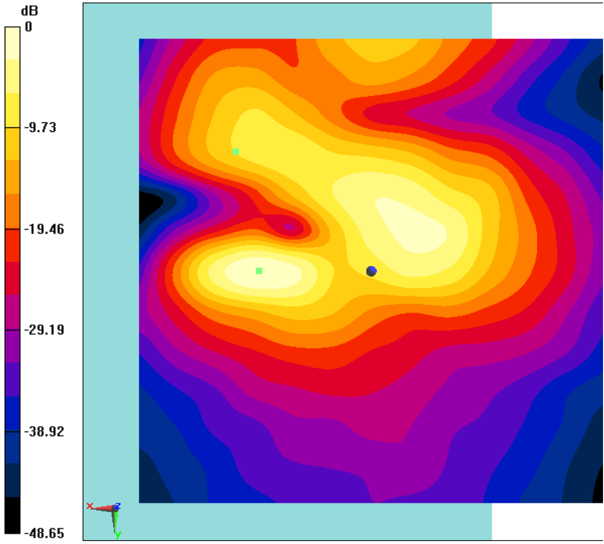
Fig B.19 T-Coil LTE B66
