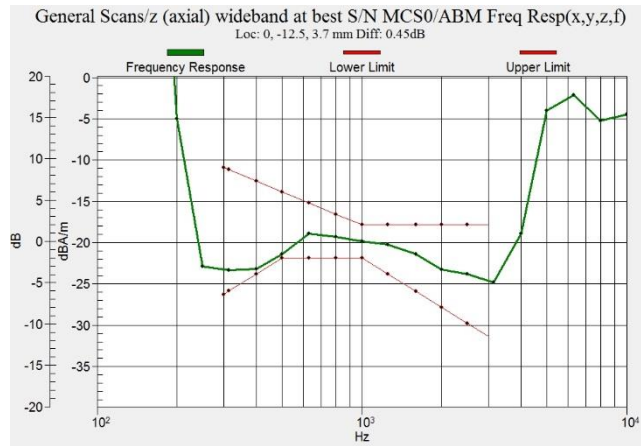
Figure C.13 Frequency Response of WiFi-5G
