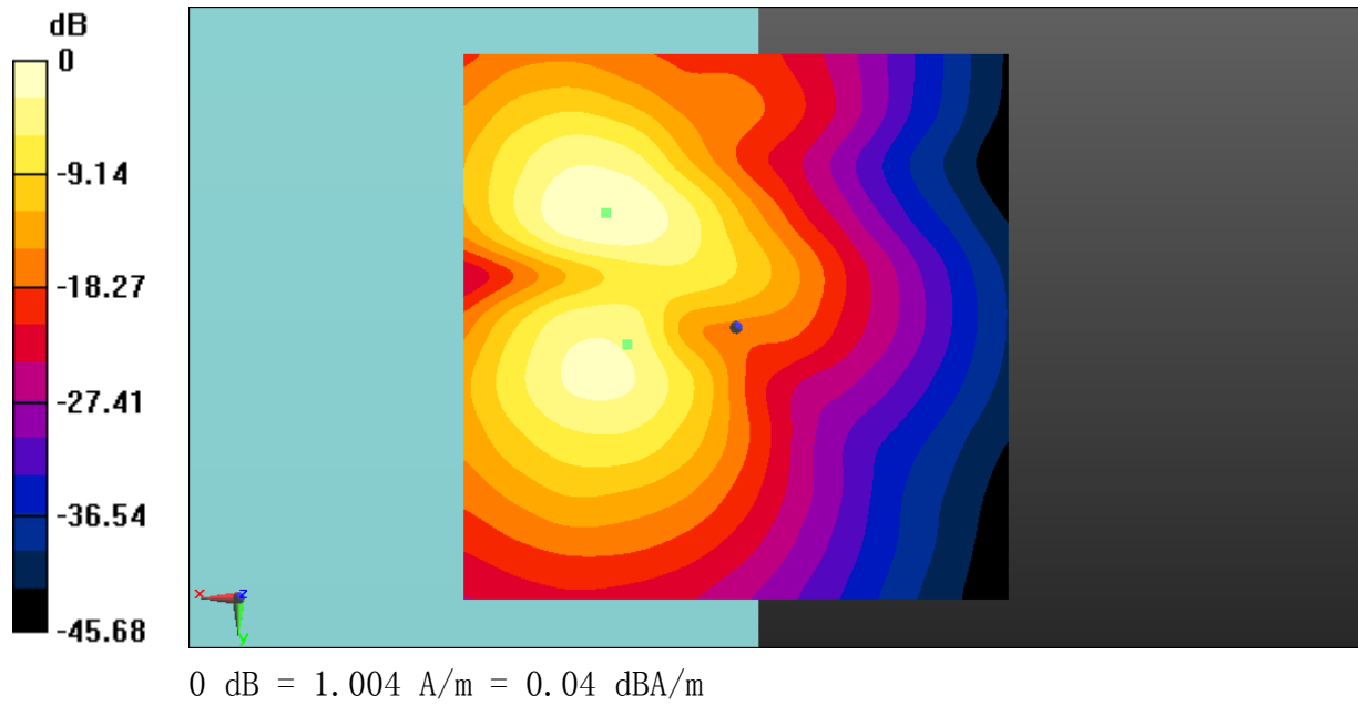
Fig B.13 T-Coil LTE B4
