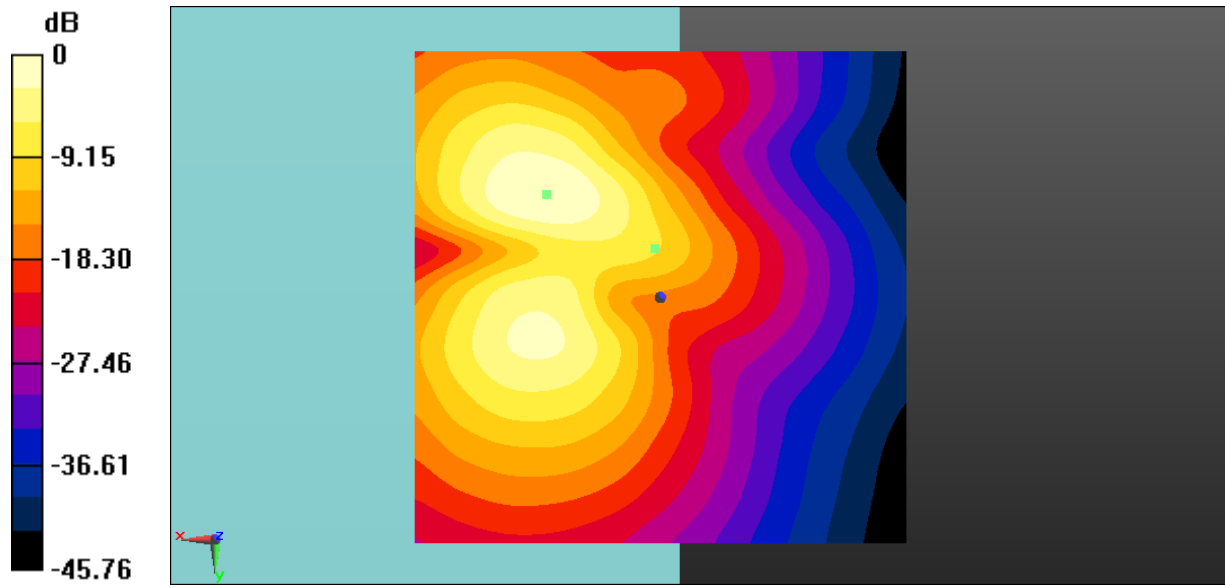
Fig B.11 T-Coil LTE B2
