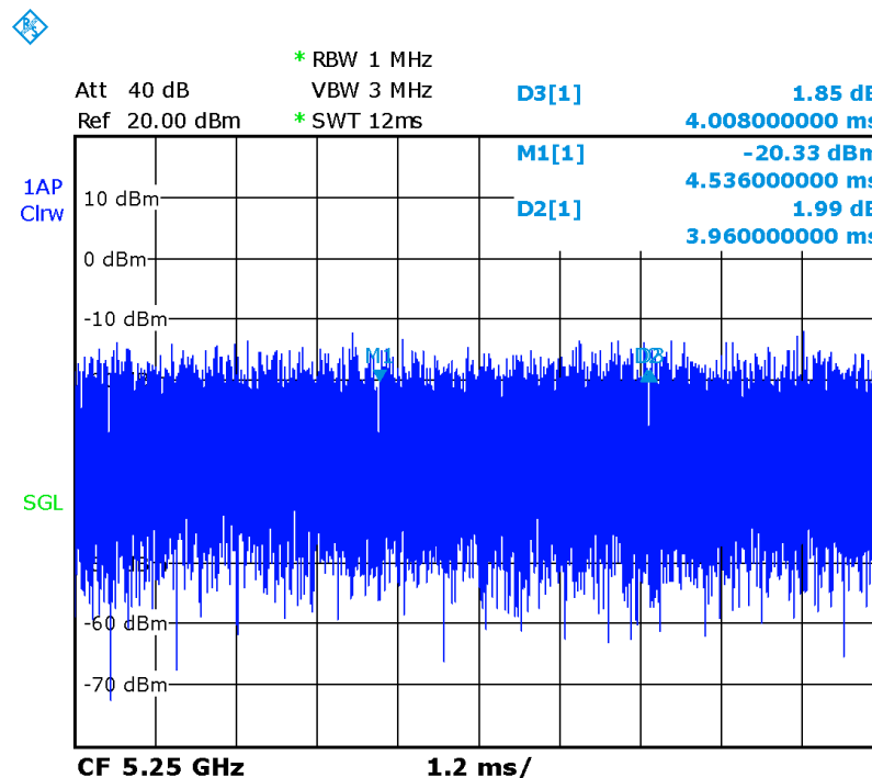
Picture 13.5 Duty factor plot for 5G
