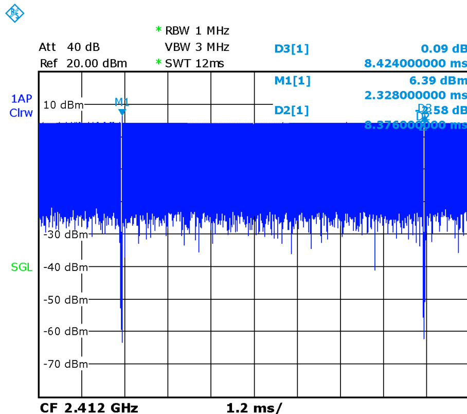
Picture 13.2 Duty factor plot for 2.4G
