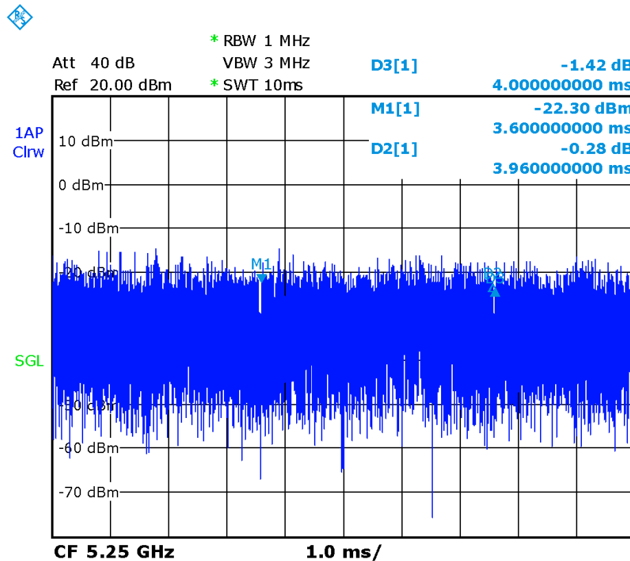
Picture 13.4 Duty factor plot for 5G
