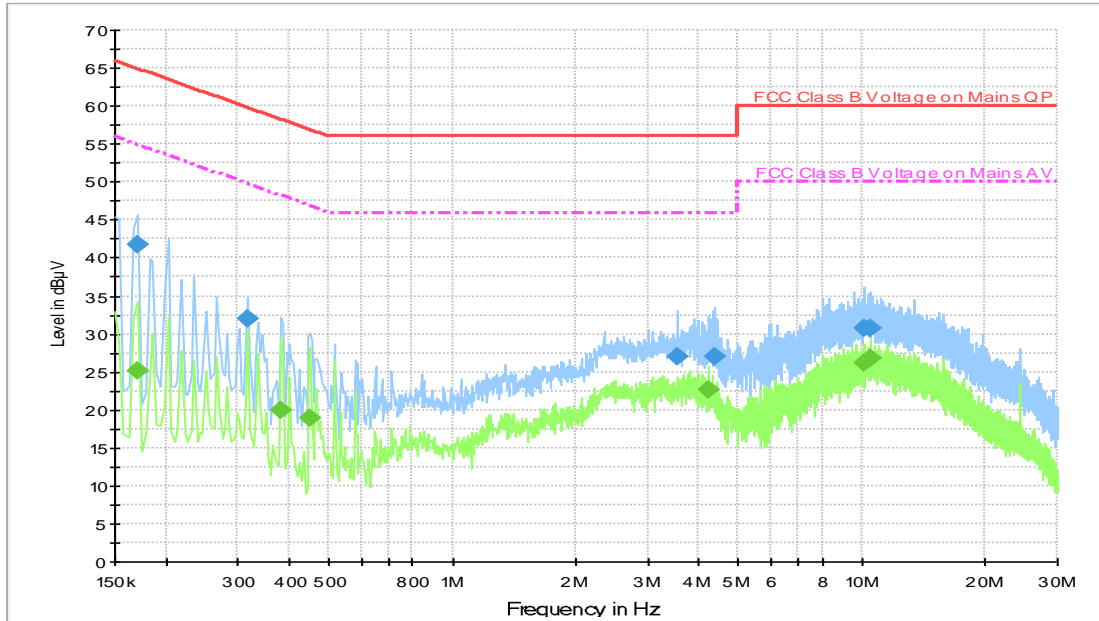
Fig.C.2.1 AC Power line Conducted Emission- Bluetooth
