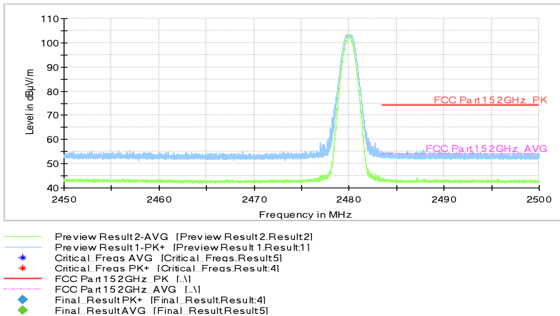
Fig.2. Frequency Band Edges: GFSK, Channel 78, 2.45 GHz - 2.50GHz
