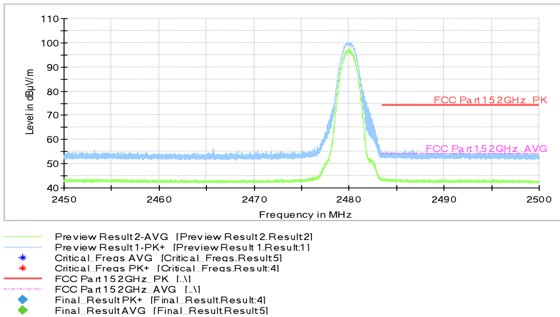
Fig.6. Frequency Band Edges: 8DPSK, Channel 78, 2.45 GHz - 2.50GHz
