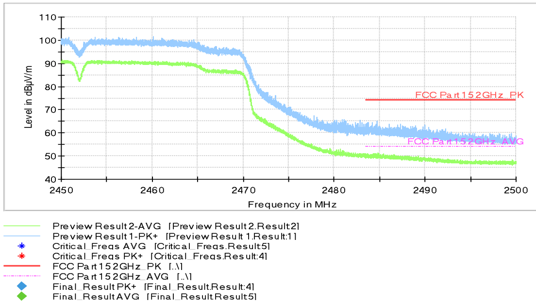
Fig.C.1.3.14 Transmitter Spurious Emission - Radiated (Power): 802.11ax-HT40, ch9, 2.45 GHz - 2.50GHz
