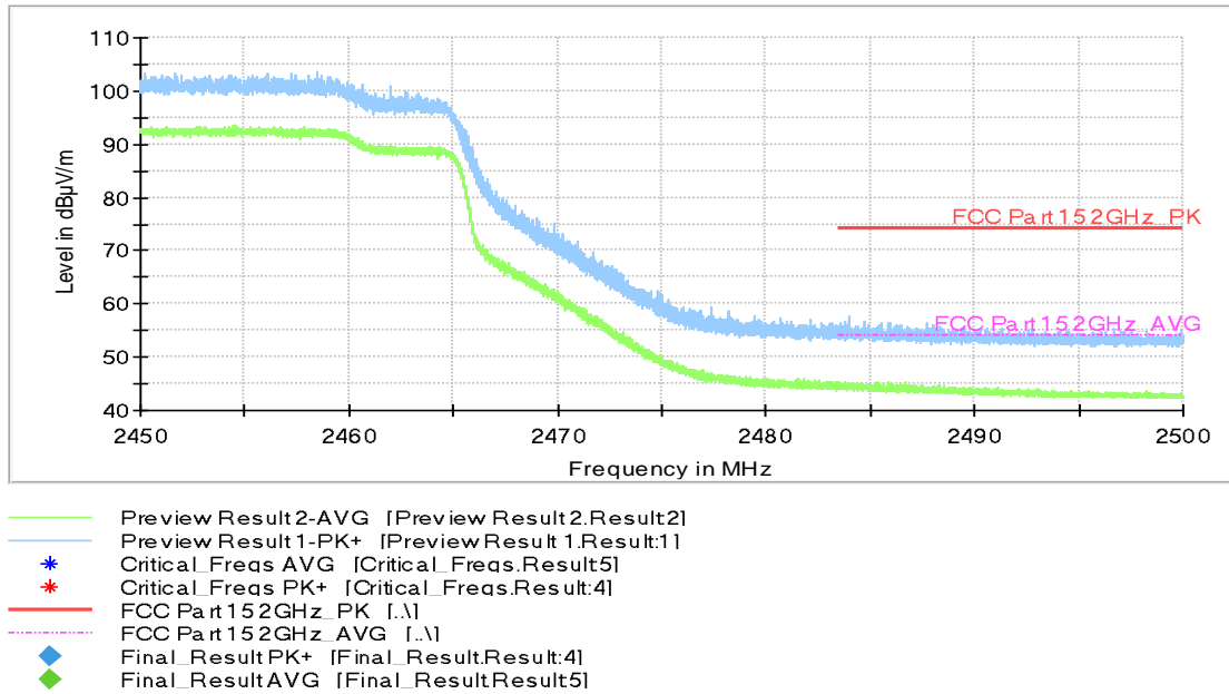
Fig.C.1.3.13 Transmitter Spurious Emission - Radiated (Power): 802.11ax-HT40, ch8, 2.45 GHz - 2.50GHz
