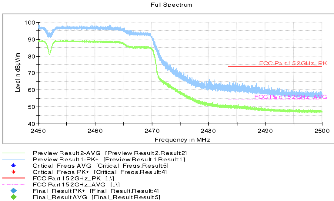
Fig.C.1.3.9 Transmitter Spurious Emission - Radiated (Power): 802.11n-HT40, ch9, 2.45 GHz - 2.50GHz
