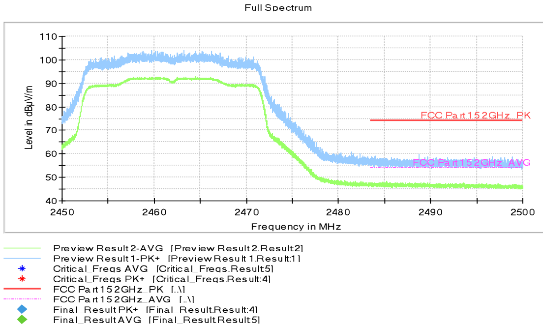
Fig.C.1.3.11 Transmitter Spurious Emission - Radiated (Power): 802.11ax-HT20, ch11, 2.45 GHz - 2.50GHz
