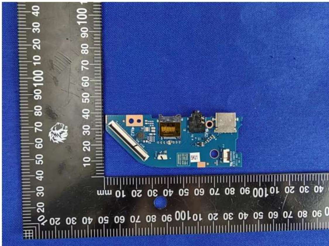
SECONDARY BOARD REAR VIEW
