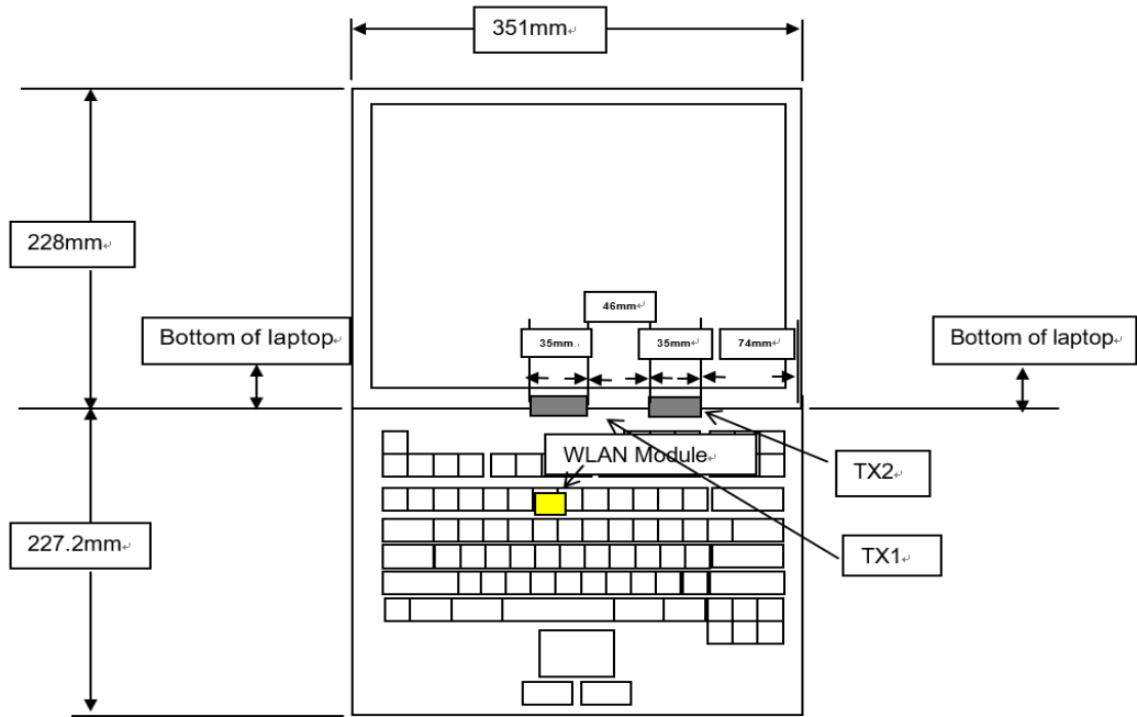
Picture 4 Antenna Locations
