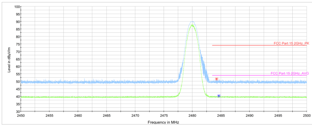
Fig.10. Frequency Band Edges: \pi/4 DQPSK, Channel 78, Hopping Off, 2.45 GHz - 2.50GHz
