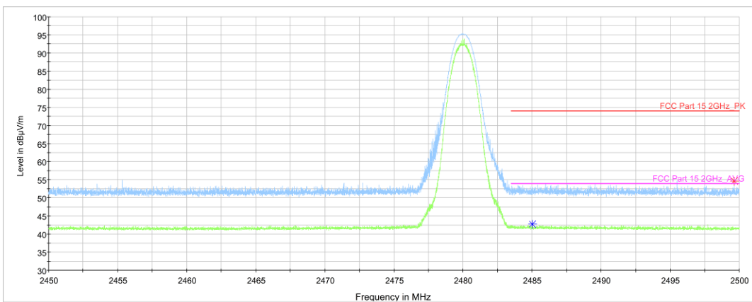
Fig.6. Frequency Band Edges: 8DPSK, Channel 78, 2.45 GHz - 2.50GHz
