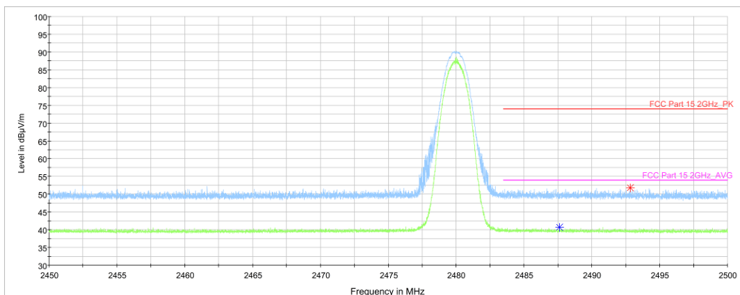
Fig.12. Frequency Band Edges: 8DPSK, Channel 78, 2.45 GHz - 2.50GHz
