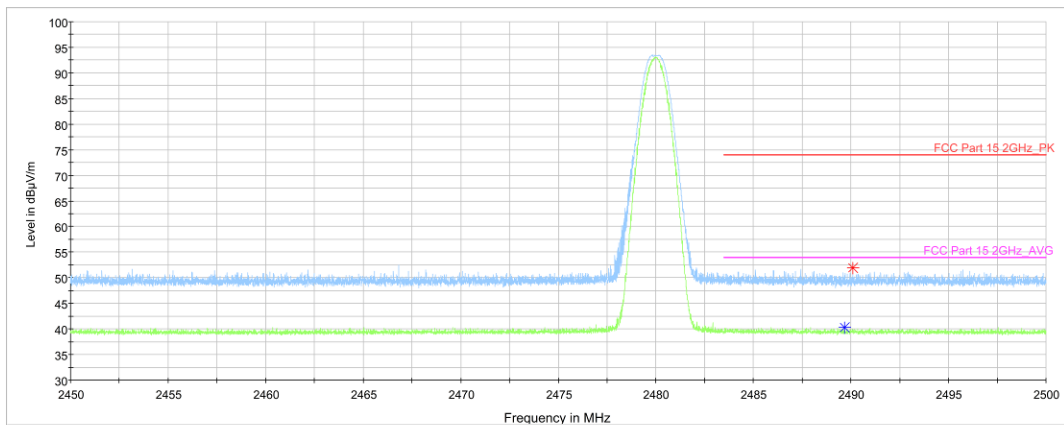
Fig.8. Frequency Band Edges: GFSK, Channel 78, Hopping Off, ch11, 2.45 GHz - 2.50GHz
