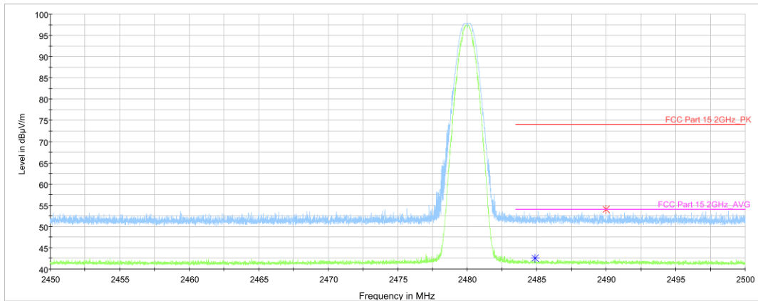
Fig.2. Frequency Band Edges: GFSK, Channel 78, Hopping Off, ch11, 2.45 GHz - 2.50GHz
