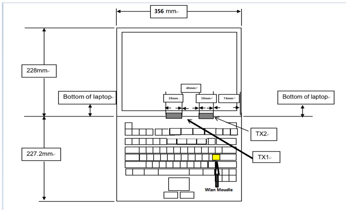
Picture 4 Antenna Locations
