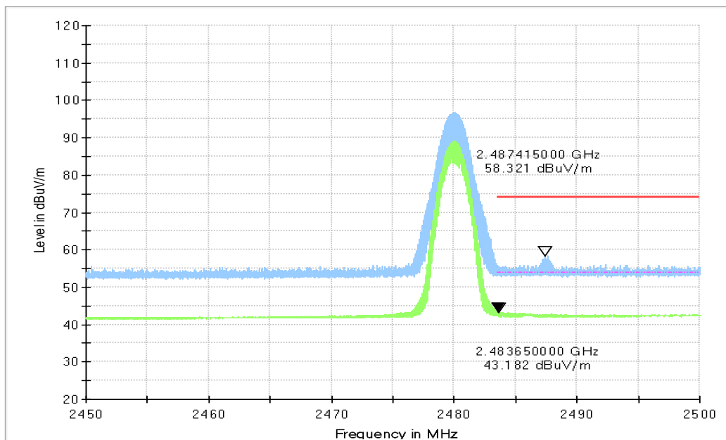
Fig.6. Frequency Band Edges: 8DPSK, Channel 78, 2.45 GHz - 2.50GHz
