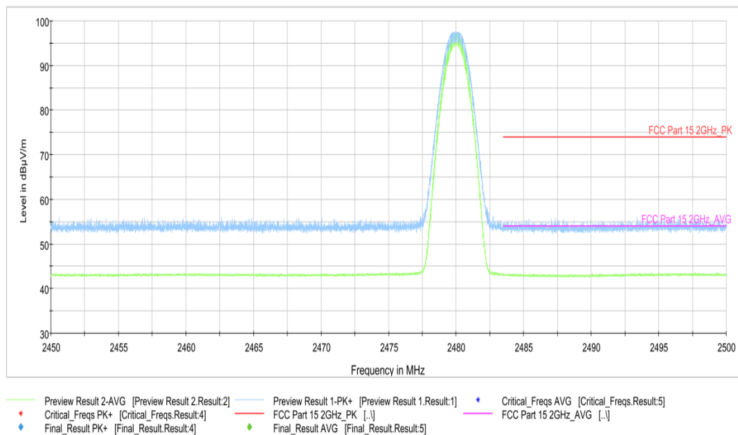
Fig.8. Frequency Band Edges: GFSK, Channel 78, Hopping Off, 2.45 GHz - 2.50GHz
