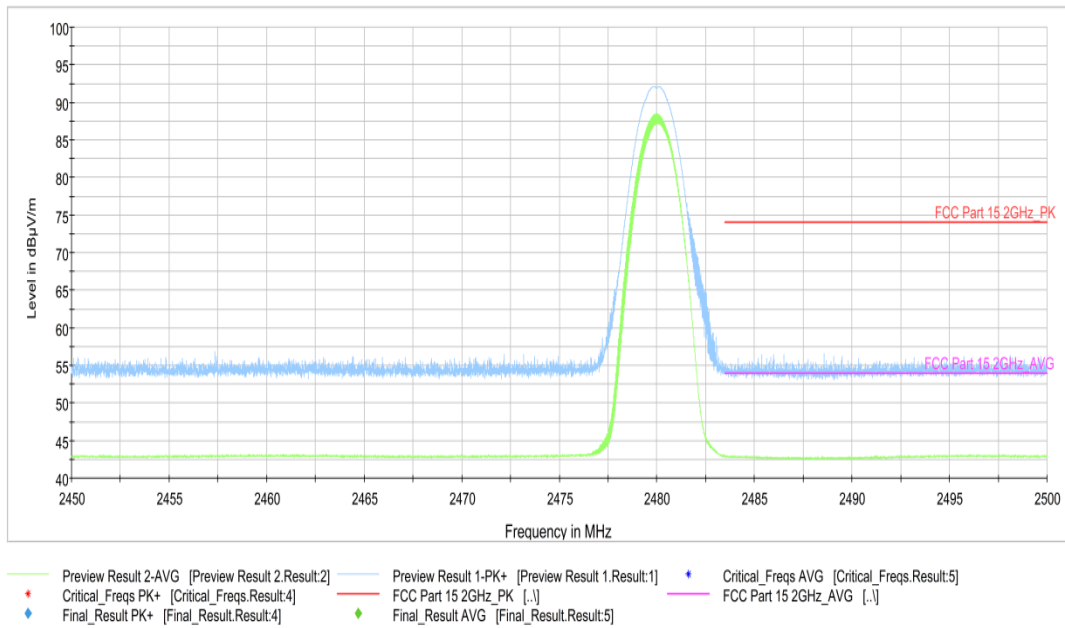
Fig.4. Frequency Band Edges: \pi/4 DQPSK, Channel 78, 2.45 GHz - 2.50GHz
