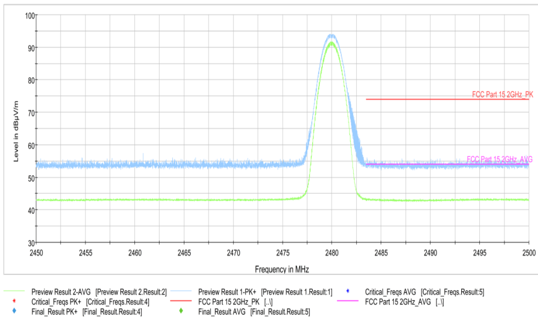
Fig.10. Frequency Band Edges: \pi/4 DQPSK, Channel 78, Hopping Off, 2.45 GHz - 2.50GHz
