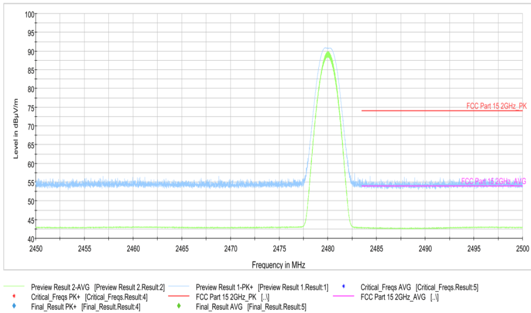
Fig.2. Frequency Band Edges: GFSK, 2480 MHz, 2.45 GHz - 2.50GHz
