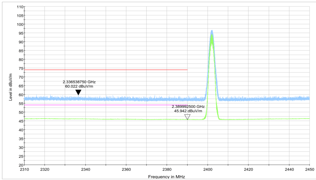
Fig.9. Frequency Band Edges: \pi/4 DQPSK, Channel 0, Hopping Off, 2.31 GHz - 2.45GHz
