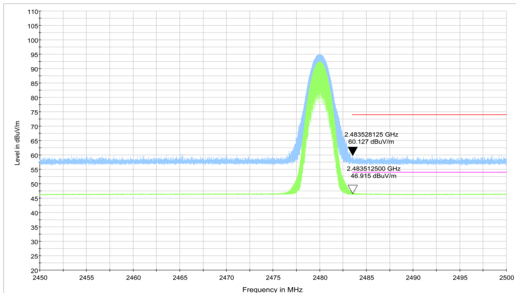
Fig.12. Frequency Band Edges: 8DPSK, Channel 78, 2.45 GHz - 2.50GHz
