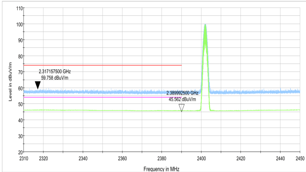
Fig.1. Frequency Band Edges: GFSK, Channel 0, 2.31 GHz – 2.45GHz
