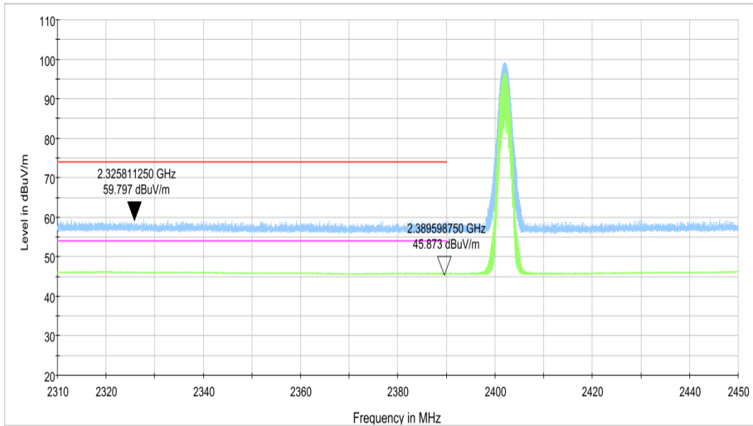
Fig.5. Frequency Band Edges: 8DPSK, Channel 0, 2.31 GHz - 2.45GHz
