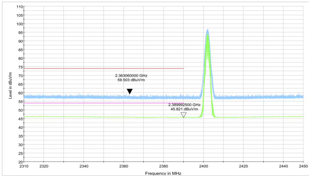
Fig.11. Frequency Band Edges: 8DPSK, Channel 0, 2.31 GHz - 2.45GHz
