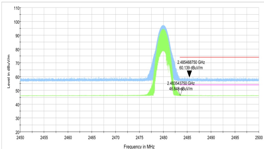
Fig.6. Frequency Band Edges: 8DPSK, Channel 78, 2.45 GHz - 2.50GHz
