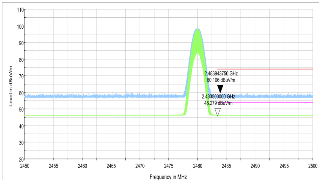
Fig.2. Frequency Band Edges: GFSK, Channel 78, 2.45 GHz - 2.50GHz
