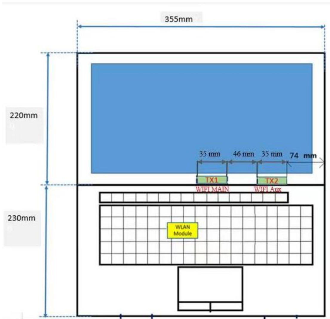
Picture 3 Antenna Locations
