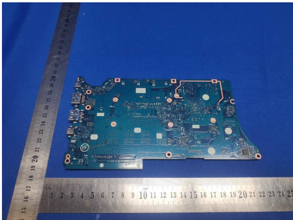
PWB view
