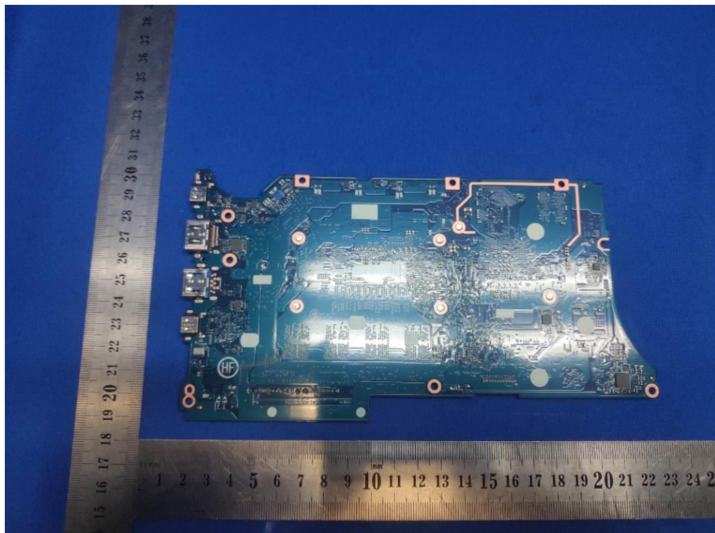
PWB view
