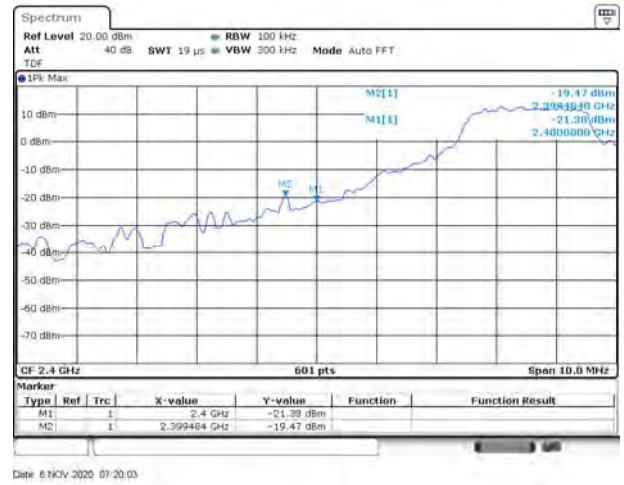
802.11ax-20 MHz (RU26) LOW CHANNEL, Reference level
