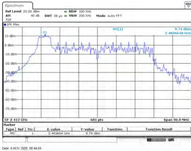
802.11ax-20 MHz (RU26) LOW CHANNEL, Carrier level
