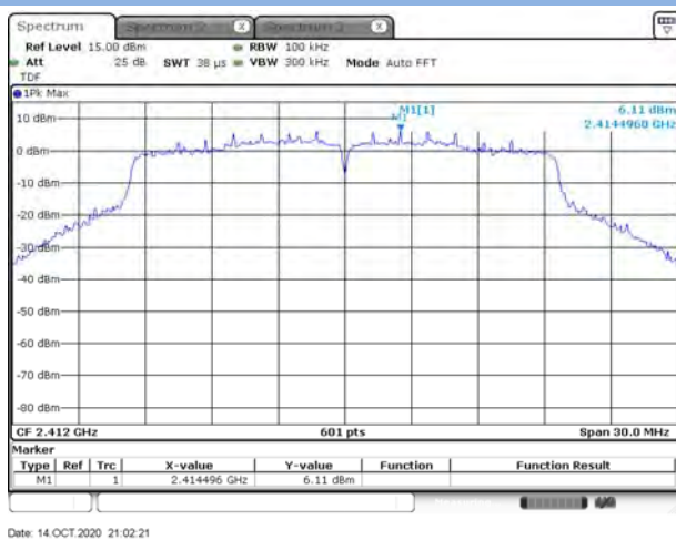
802.11ax-20 MHz (SU) LOW CHANNEL, Carrier level
