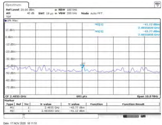
802.11ax-20 MHz (RU26) HIGH CHANNEL, Reference level
