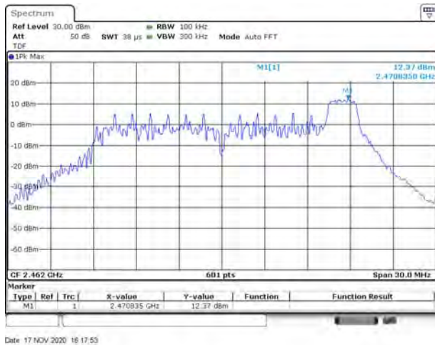
802.11ax-20 MHz (RU26) HIGH CHANNEL, Carrier level
