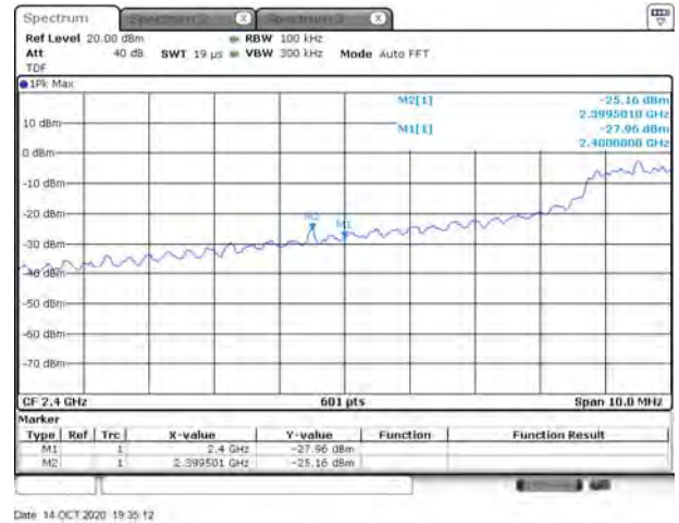
802.11n-40 MHz LOW CHANNEL, Reference level
