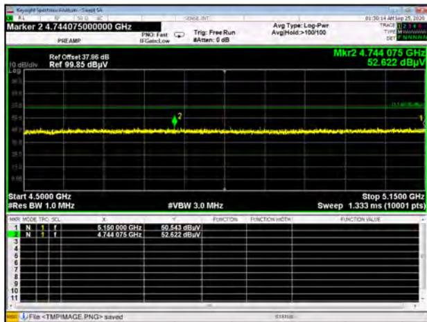
U-NII-2A 11ax20 CH52 Peak
