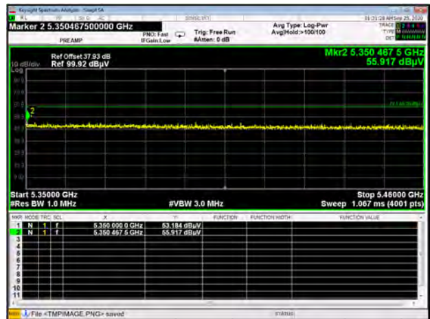
U-NII-2A 11ax20 CH64 Peak
