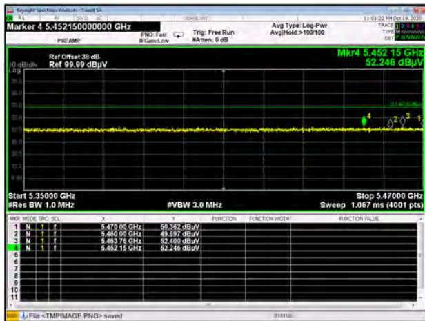
U-NII-2C 11ax20 CH144 Peak
