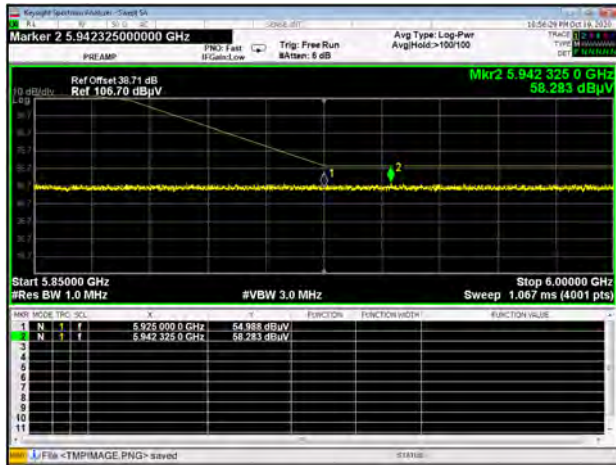
U-NII-3 11ax80 CH138 Peak
