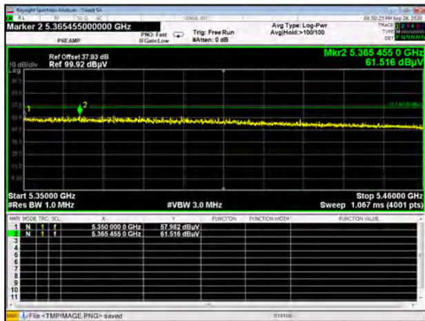
U-NII-2A 11ax160 CH50 Peak
