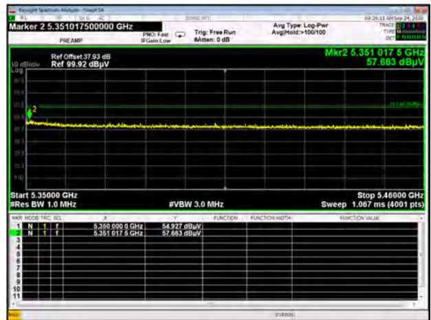
U-NII-2A 11ax40 CH62 Peak
