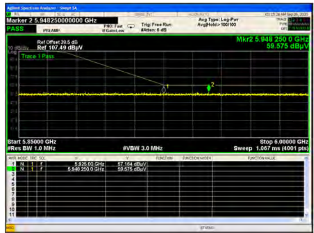
U-NII-3 11n40 CH159 Peak
