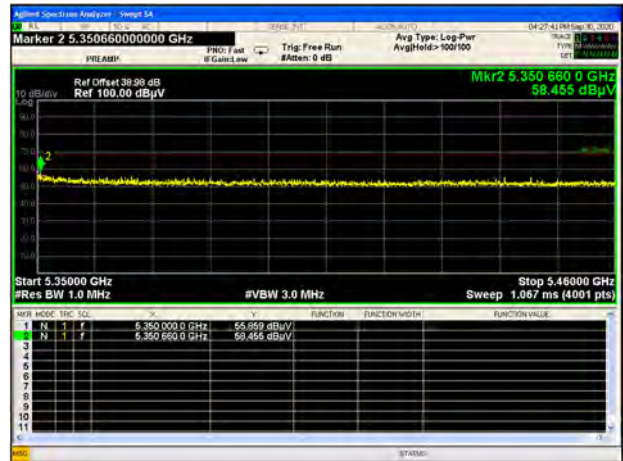
U-NII-2A 11ac20 CH64 Peak
