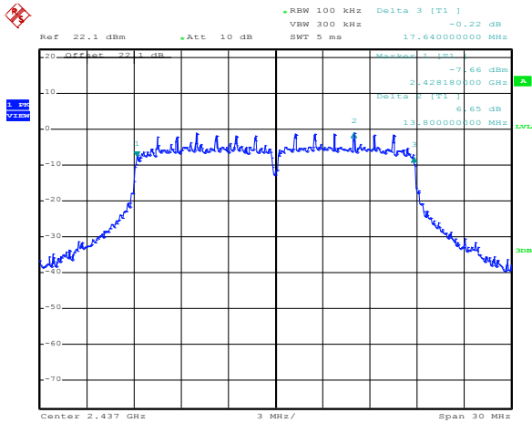
Figure 8.2-3: 6 dB bandwidth on 802.11g, min rate, sample plot
