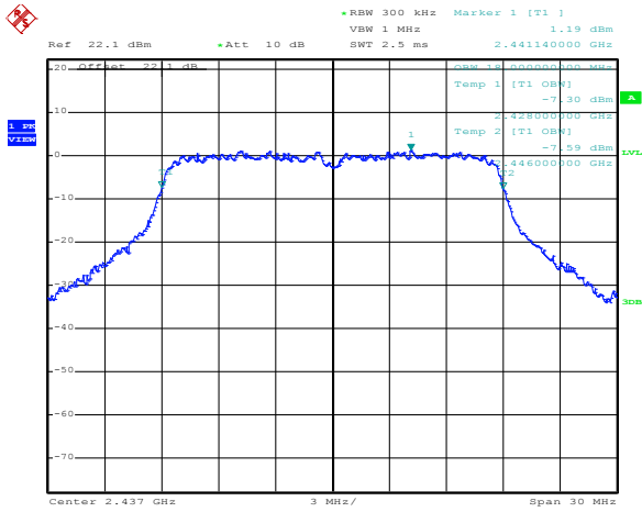
Figure 8.3-3: 99 % bandwidth on 802.11g, min rate, sample plot
