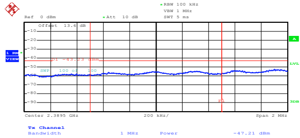
Figure 8.5-42: Conducted average lower band edge emission for 802.11g at minimum rate
