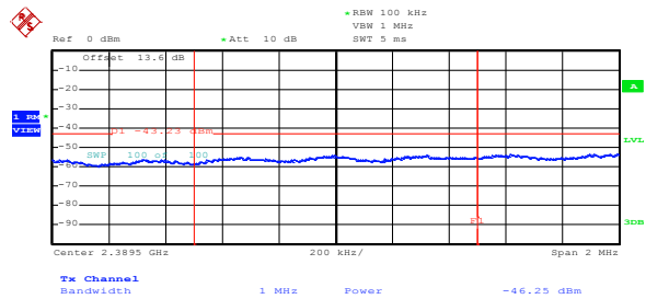
Figure 8.5-44: Conducted average lower band edge emission for 802.11g at maximum rate
