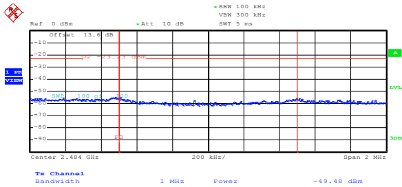
Figure 8.5-49: Conducted peak upper band edge emission for 802.11b at minimum rate
