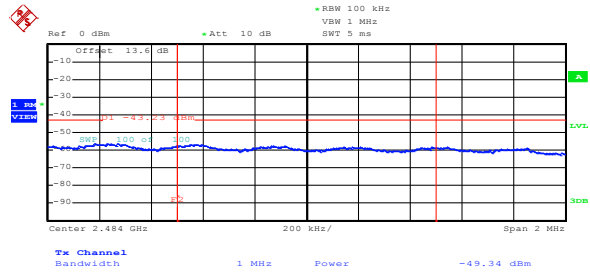
Figure 8.5-60: Conducted average upper band edge emission for 802.11n at maximum rate
