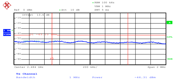
Figure 8.5-58: Conducted average upper band edge emission for 802.11n at minimum rate
