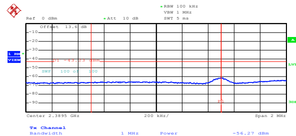
Figure 8.5-38: Conducted average lower band edge emission for 802.11b at minimum rate
