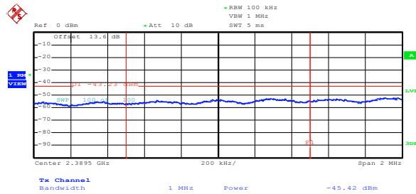
Figure 8.5-48: Conducted average lower band edge emission for 802.11n at maximum rate
