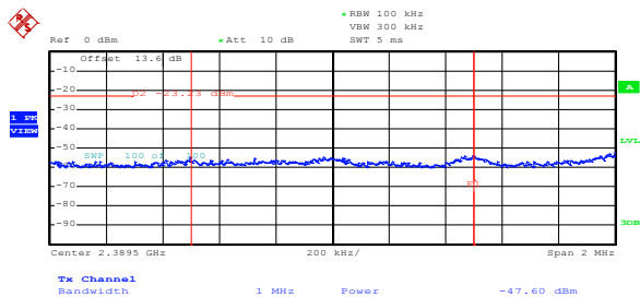
Figure 8.5-37: Conducted peak lower band edge emission for 802.11b at minimum rate
