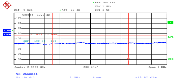
Figure 8.5-40: Conducted average lower band edge emission for 802.11b at maximum rate
