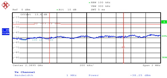
Figure 8.5-41: Conducted peak lower band edge emission for 802.11g at minimum rate
