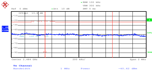
Figure 8.5-59: Conducted peak upper band edge emission for 802.11n at maximum rate
