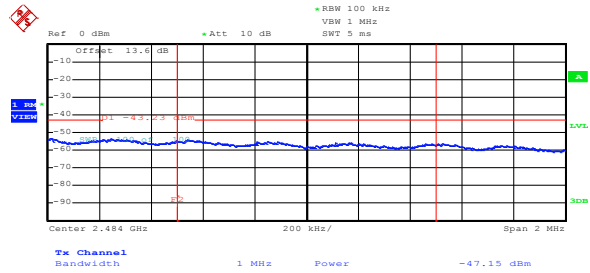
Figure 8.5-54: Conducted average upper band edge emission for 802.11g at minimum rate
