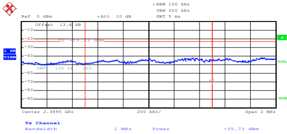
Figure 8.5-45: Conducted peak lower band edge emission for 802.11n at minimum rate
