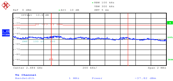
Figure 8.5-53: Conducted peak upper band edge emission for 802.11g at minimum rate
