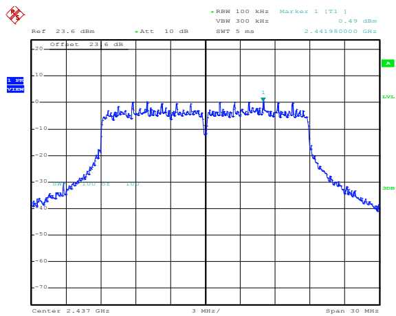
Figure 8.6-4: PSD sample plot on 802.11g at maximum rate
