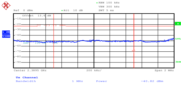
Figure 8.5-39: Conducted peak lower band edge emission for 802.11b at maximum rate
