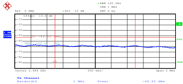
Figure 8.5-56: Conducted average upper band edge emission for 802.11g at maximum rate
