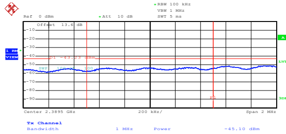
Figure 8.5-46: Conducted average lower band edge emission for 802.11n at minimum rate
