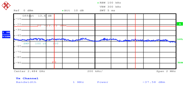
Figure 8.5-57: Conducted peak upper band edge emission for 802.11n at minimum rate
