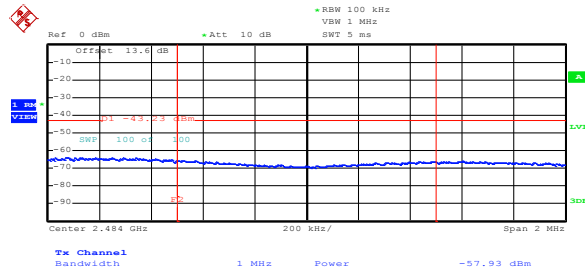
Figure 8.5-50: Conducted average upper band edge emission for 802.11b at minimum rate
