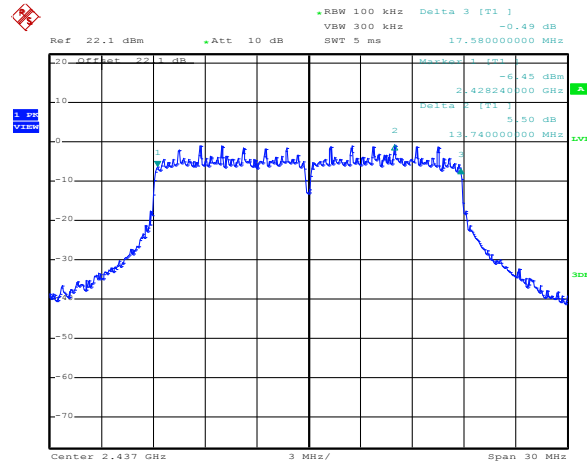
Figure 8.2-4: 6 dB bandwidth on 802.11g, max rate, sample plot
