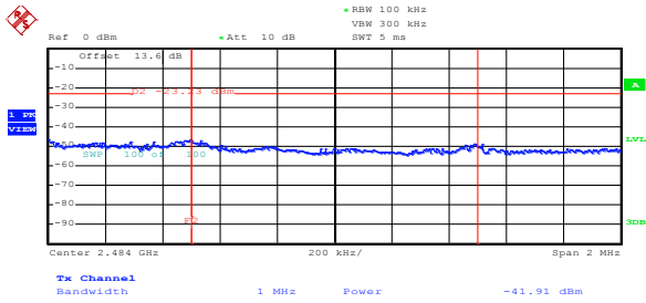
Figure 8.5-51: Conducted peak upper band edge emission for 802.11b at maximum rate
