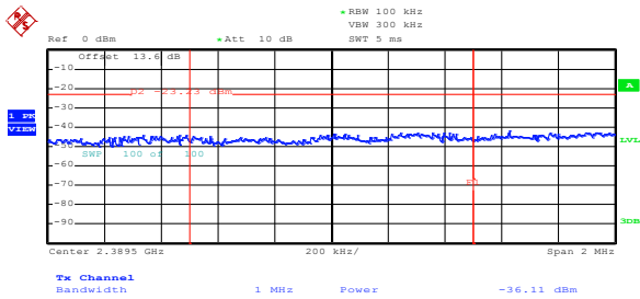
Figure 8.5-47: Conducted peak lower band edge emission for 802.11n at maximum rate
