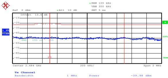
Figure 8.5-55: Conducted peak upper band edge emission for 802.11g at maximum rate
