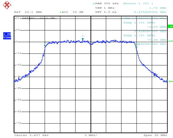
Figure 8.3-4: 99 % bandwidth on 802.11g, max rate, sample plot
