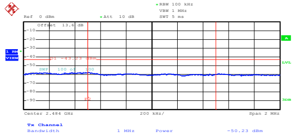
Figure 8.5-52: Conducted average upper band edge emission for 802.11b at maximum rate
