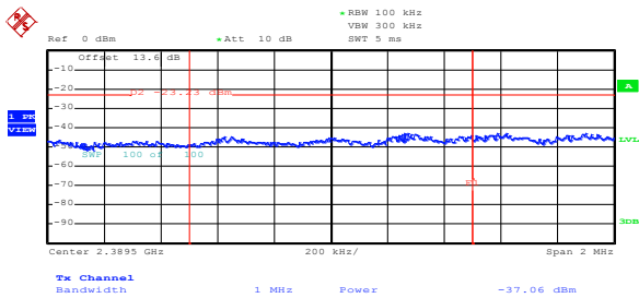
Figure 8.5-43: Conducted peak lower band edge emission for 802.11g at maximum rate
