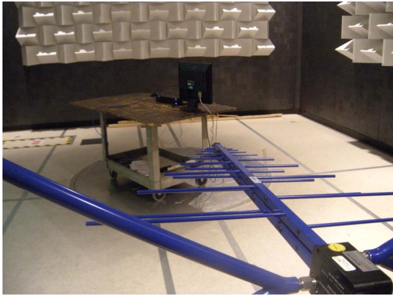
Photo 5 Test Setup – Radiated Emissions (below 1 GHz)
