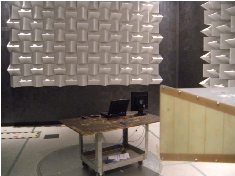
Photo 6 Test Setup – Radiated Emissions (above 1 GHz)
