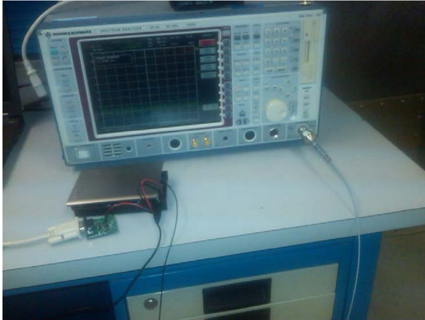
Test Setup – Conducted Emissions
