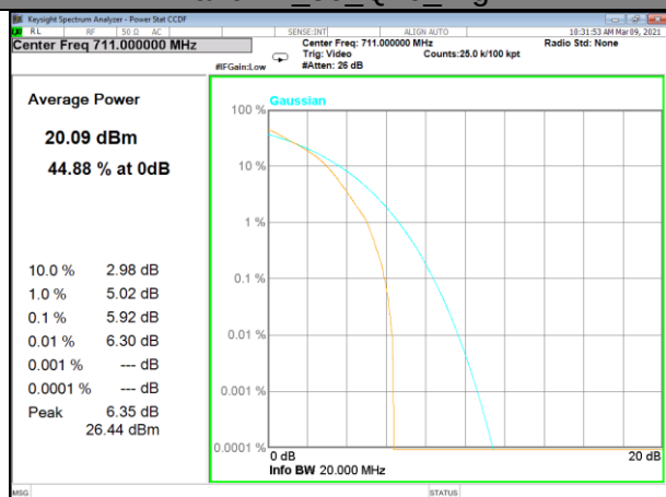
Band 12_50_Q16_High
