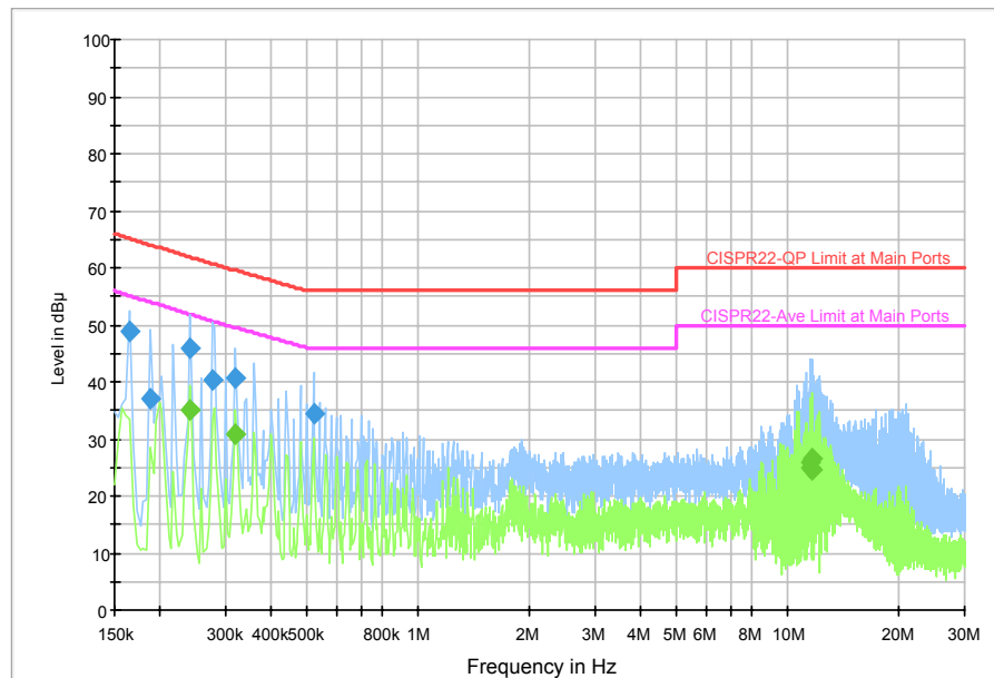
EMI_ENV216 Auto Test-L CISPR22
